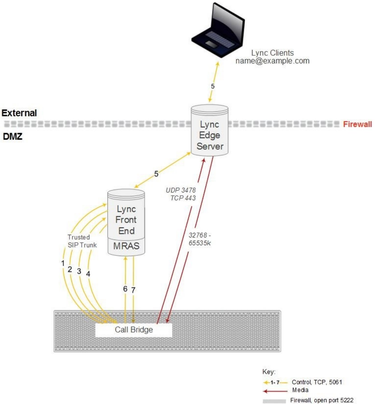
Figure 15: Call Bridge to Lync Edge server call flow
