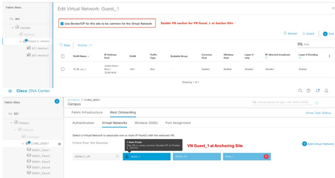
Figure 12: Anchor VN Creation and Association in Cisco DNA Center
