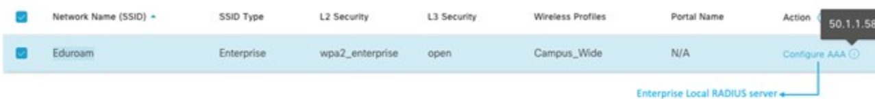
Figure 7: Eduroam SSID Configuration on Cisco DNA Center
