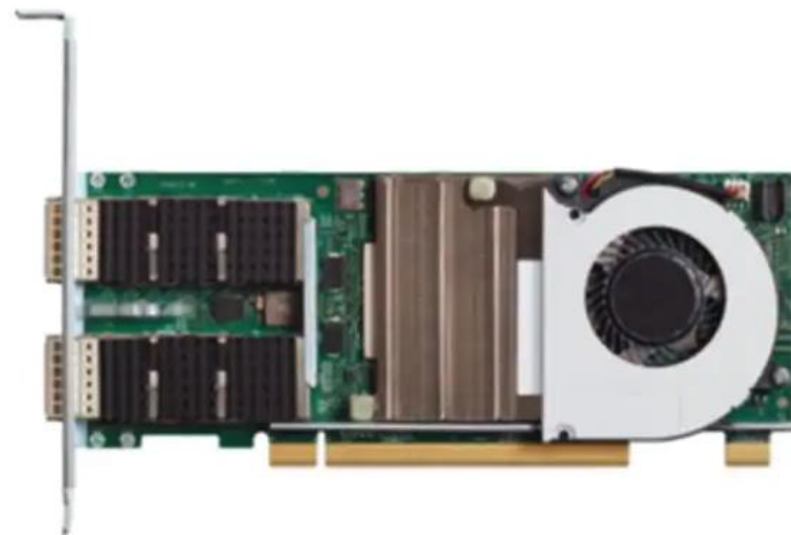
Figure 17 Cisco UCS VIC 1495
