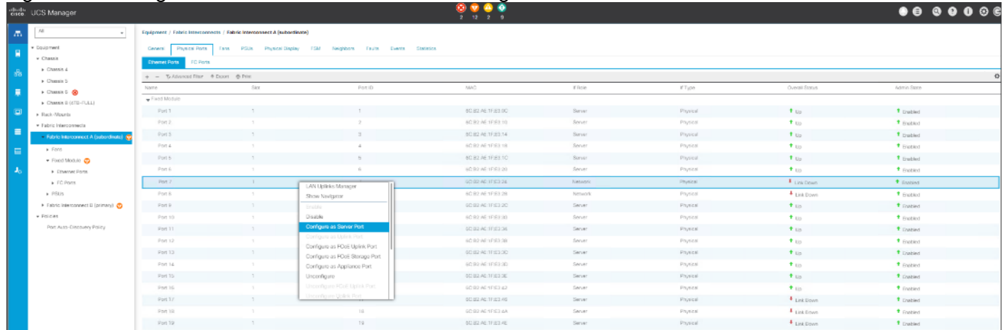
Figure 29 Configure Network Port on Cisco UCS Manager Fabric Interconnect
