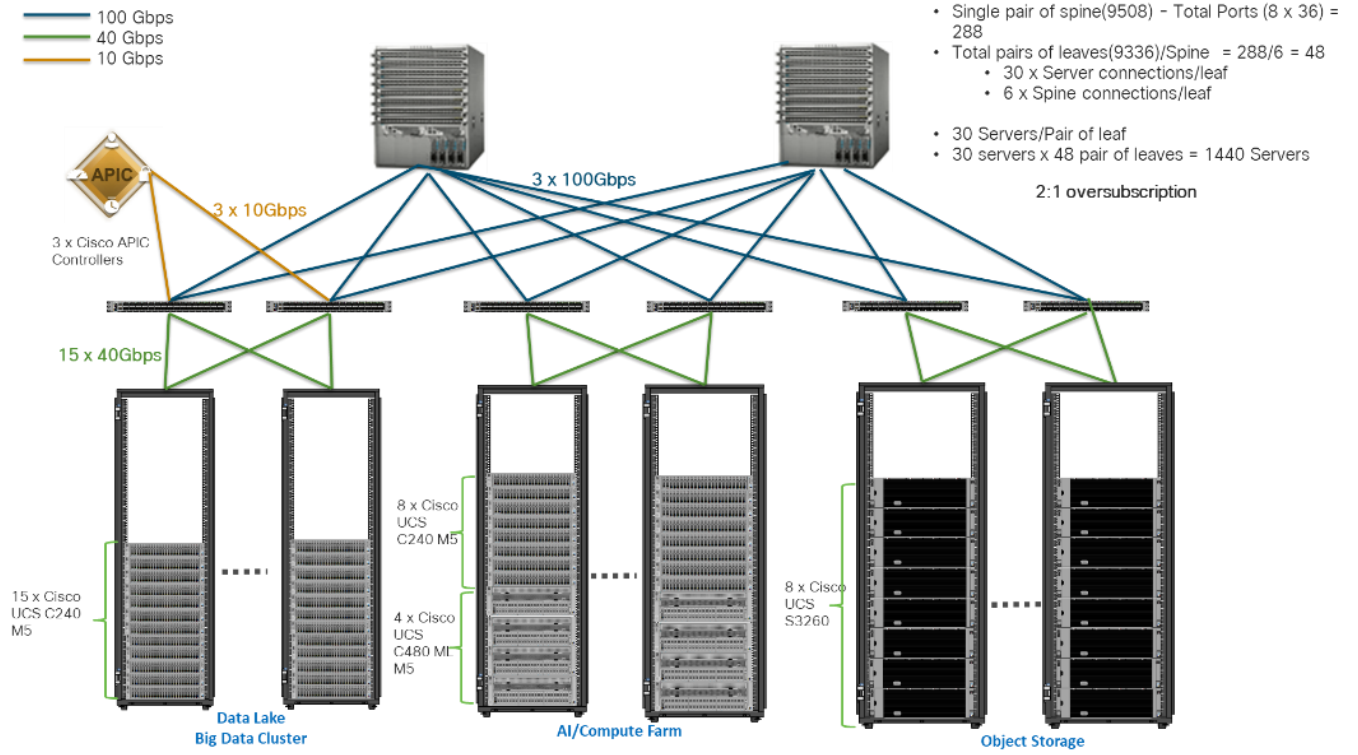
Figure 7 Scaled Architecture with 2:1 Oversubscription with Cisco ACI
