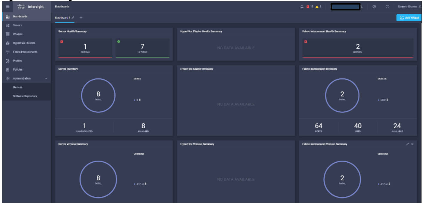
Figure 24 Intersight Dashboard
