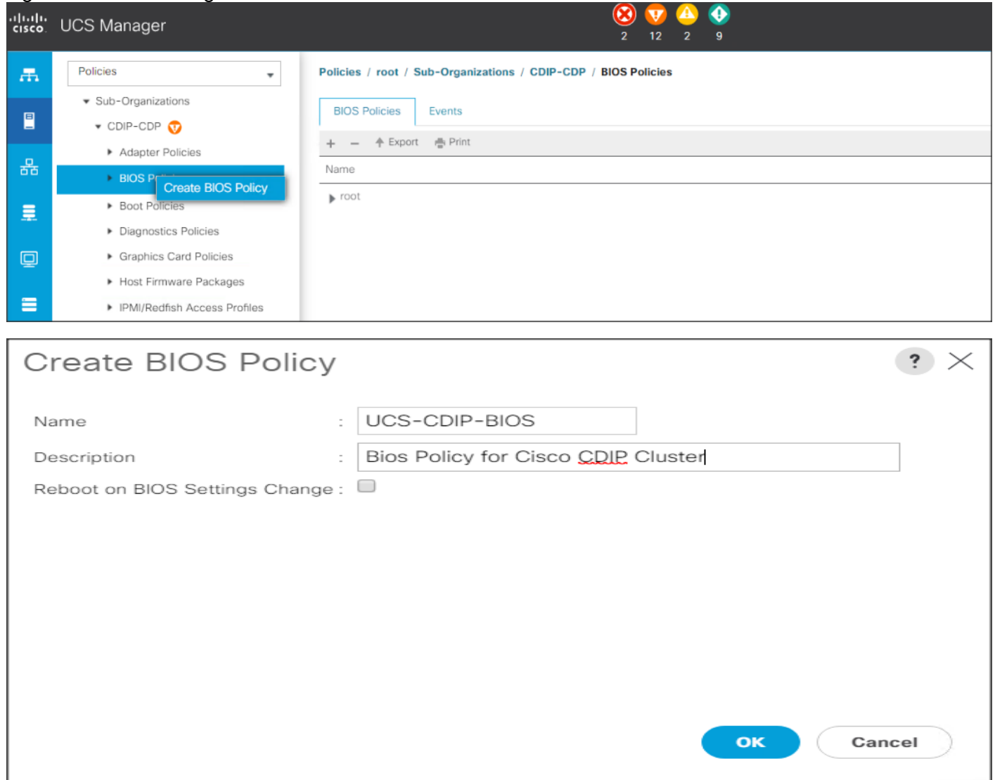
Figure 44 BIOS Configuration
