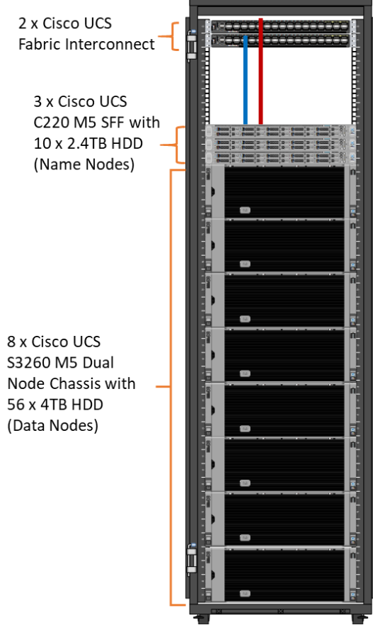
Figure 20 Cisco Data Intelligence Platform - 16 Node Configuration with CDP DC
