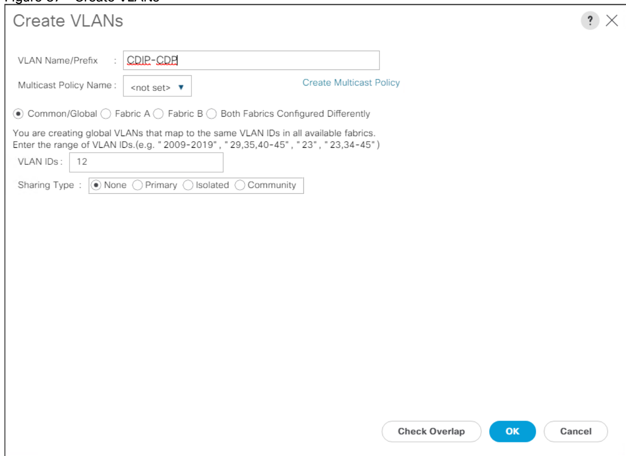
Figure 37 Create VLANs
