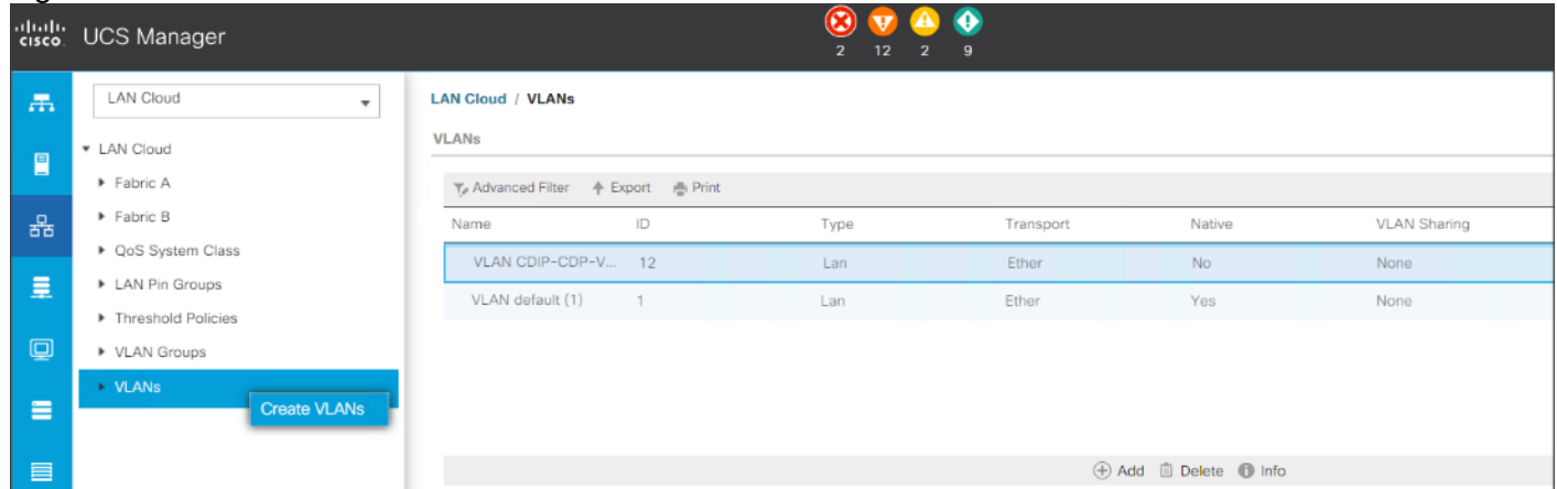
Figure 36 Create VLAN
