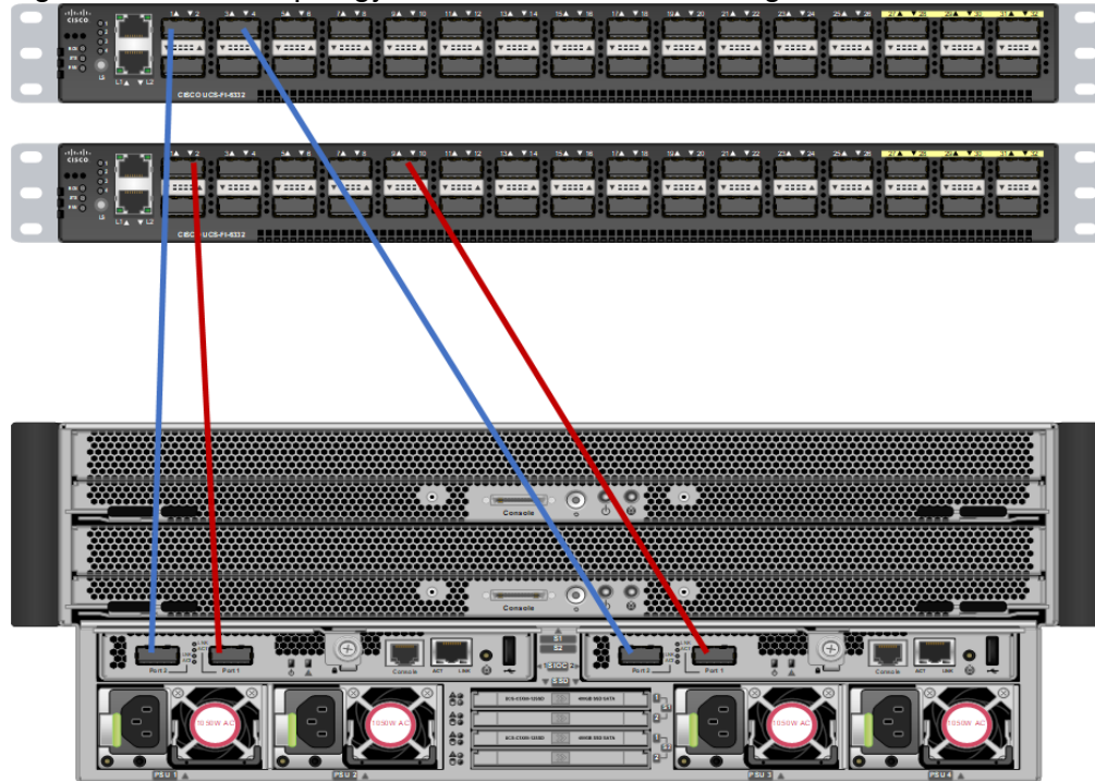
Figure 21 Fabric Topology for Cisco UCS S3260 Storage Server
