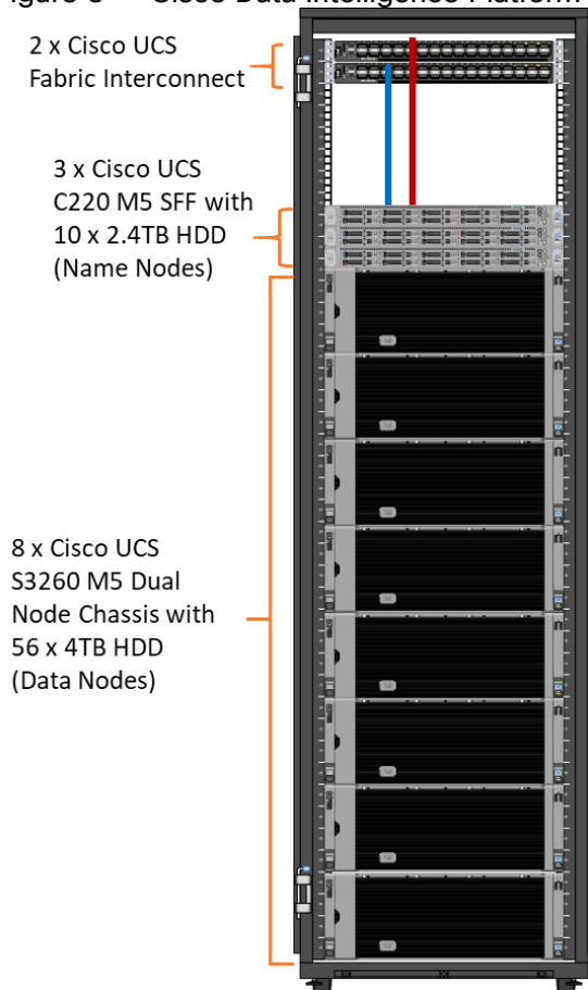
Figure 5 Cisco Data Intelligence Platform with Cloudera Data Platform Data Center – Data Lake
