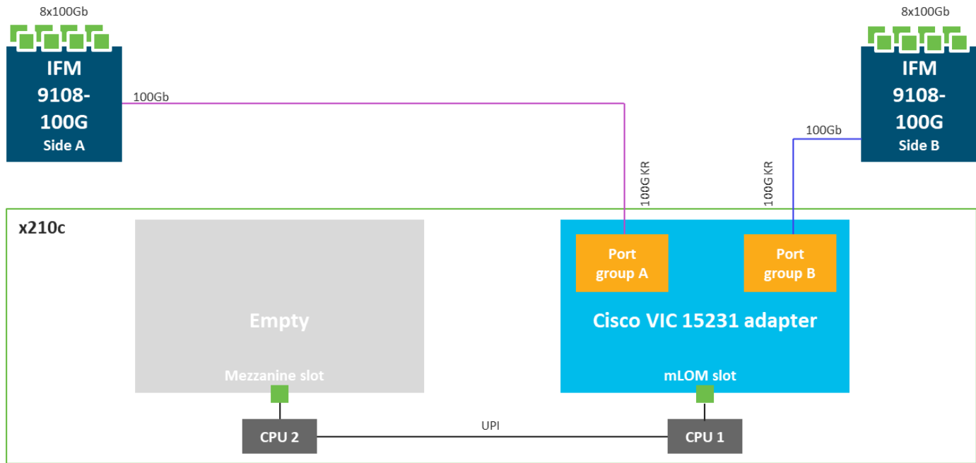
Figure 9. Cisco UCS VIC 15231 in Cisco UCS X210c M6
