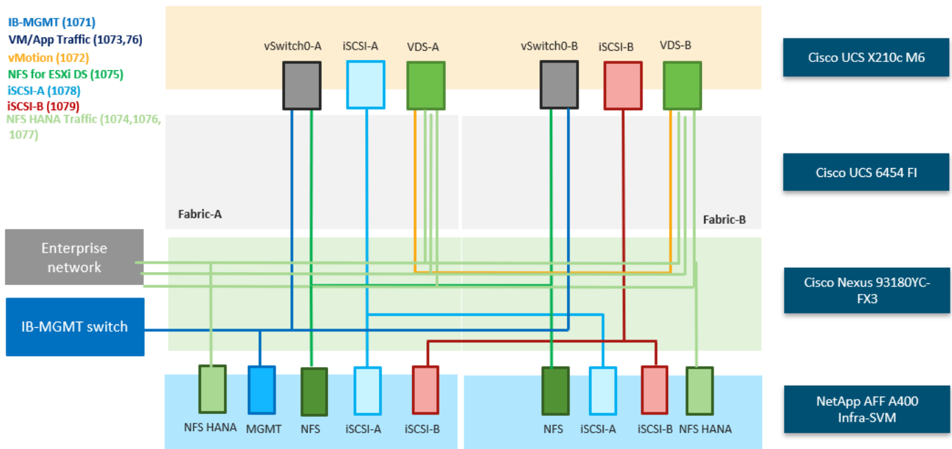
Figure 26. Logical End-to-End Connectivity for iSCSI Design
