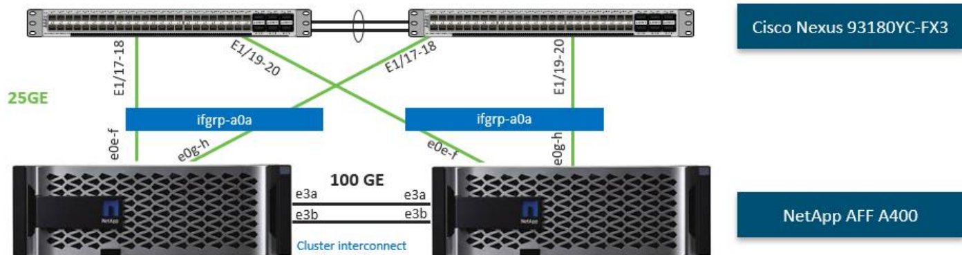
Figure 30. NetApp AFF A400 Ethernet Connectivity
