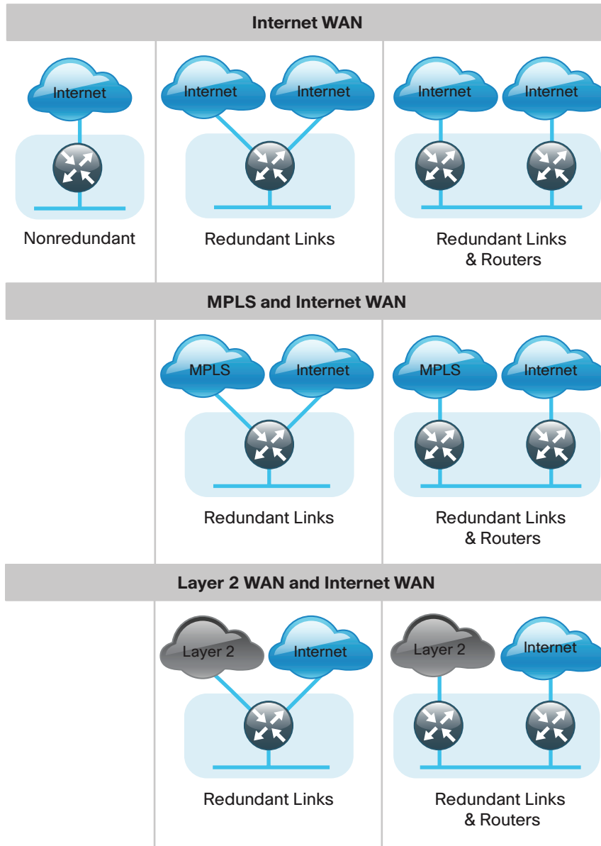
Figure 6 - WAN remote-site designs
