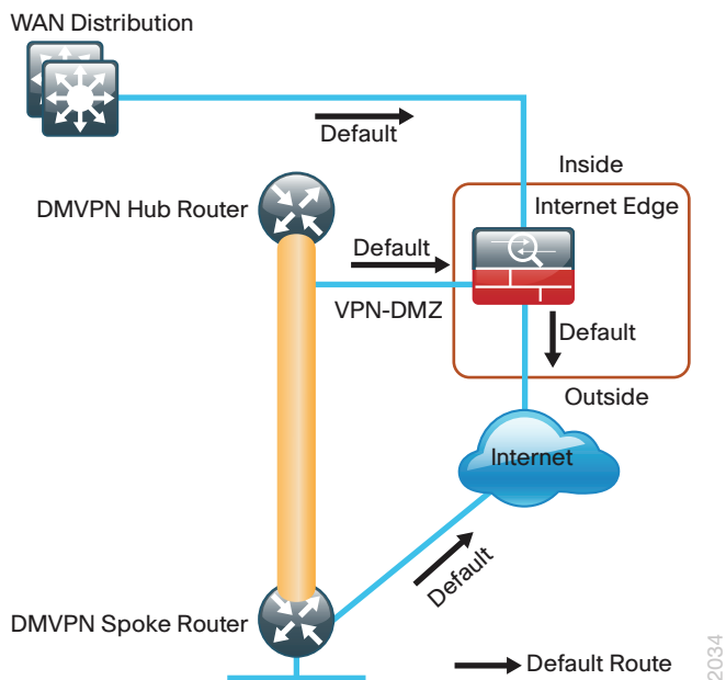
Figure 28 - IPsec tunnel
