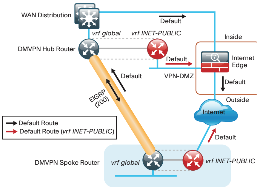
Figure 16 - Front door VRF (FVRF)
