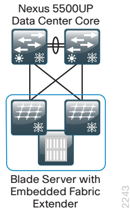
Figure 26 - Non-Cisco blade server system with embedded Cisco Nexus fabric extenders
