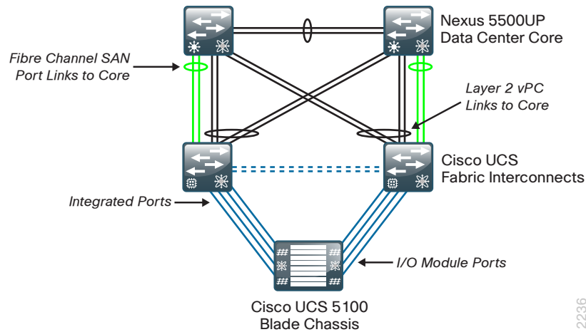
Figure 18 - Cisco UCS fabric interconnect to core
