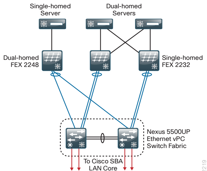
Figure 8 - Ethernet switching fabric physical connections
