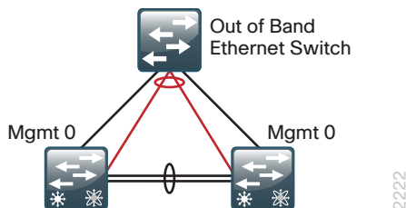
Figure 11 - Providing Layer 3 connectivity by using core Cisco Nexus 5500UP switches
