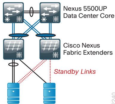
Figure 21 - Server with active/standby NIC-to-Cisco FEX connection
