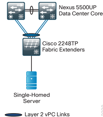
Figure 20 - Single-homed server to dual-homed Cisco FEX
