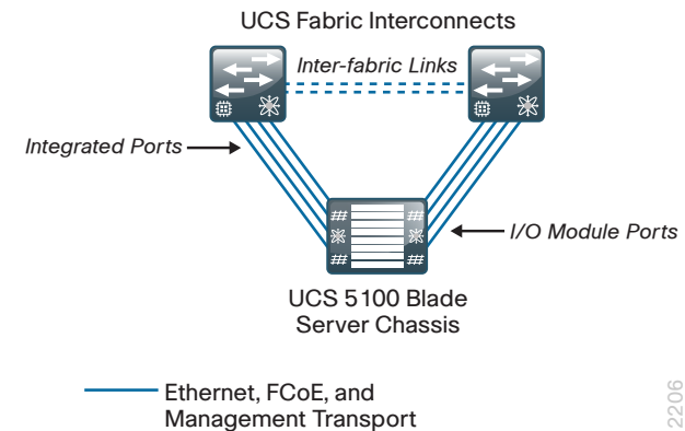
Figure 17 - Cisco UCS Blade Chassis System component connections
