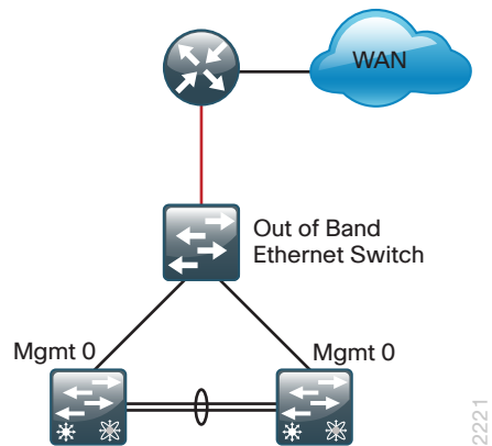
Figure 10 - WAN router providing Layer 3 connectivity
