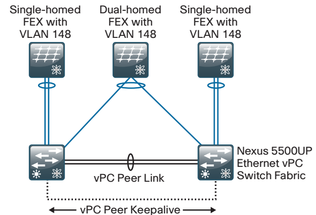
Figure 7 - Cisco FEX and vPC combined
