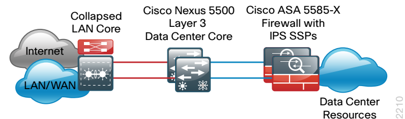
Figure 27 - Deploy firewall inline to protect data resources
