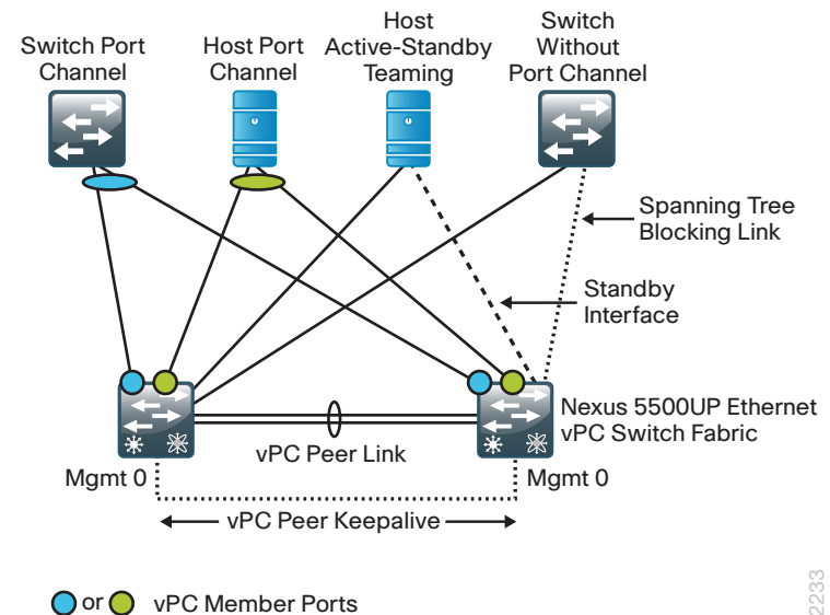
Figure 15 - vPC member and non-member ports
