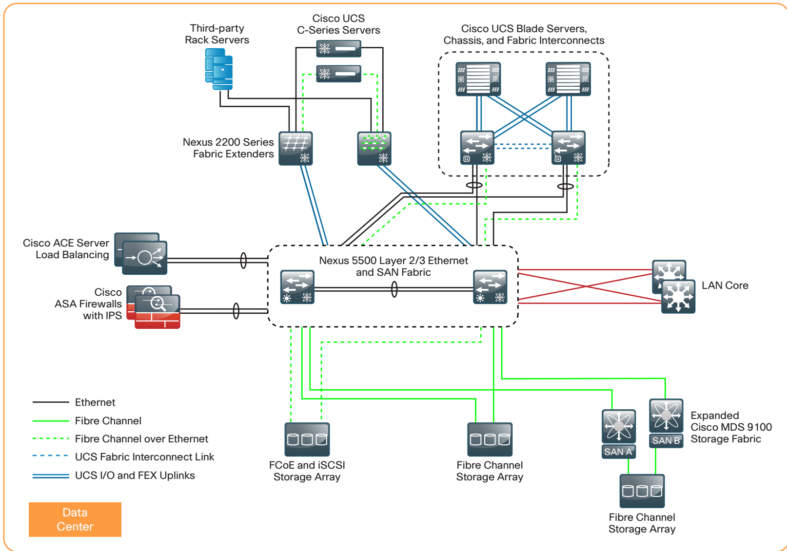
Figure 14 - Cisco SBA data center design
