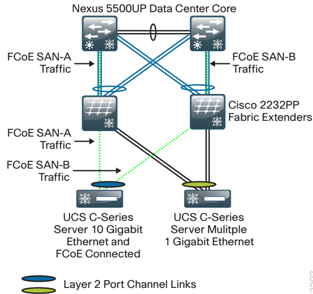
Figure 23 - Enhanced vPC with FCoE traffic
