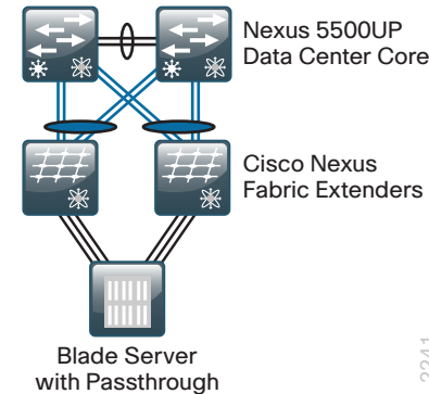
Figure 24 - Third-party blade server system with pass-through module
