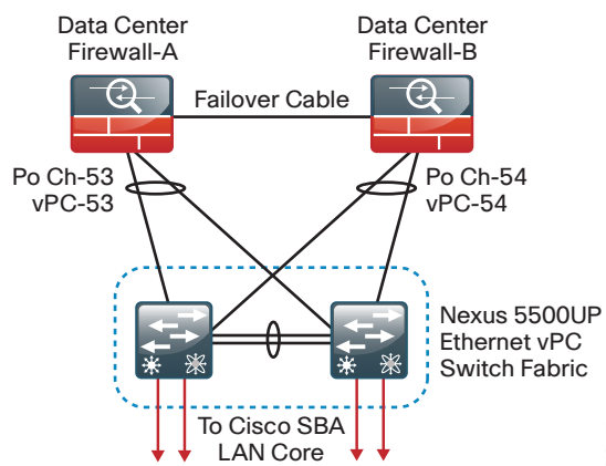
Figure 31 - Firewall to data center core switch connections
