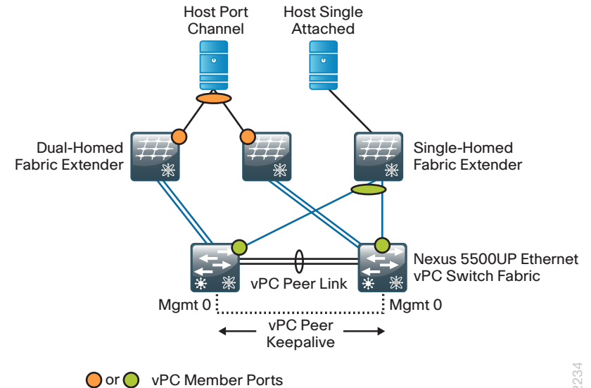
Figure 16 - Cisco Nexus FEX connectivity to data center core
