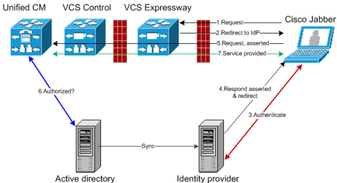
Figure 8 Remote single sign-on for on-premises UC services
