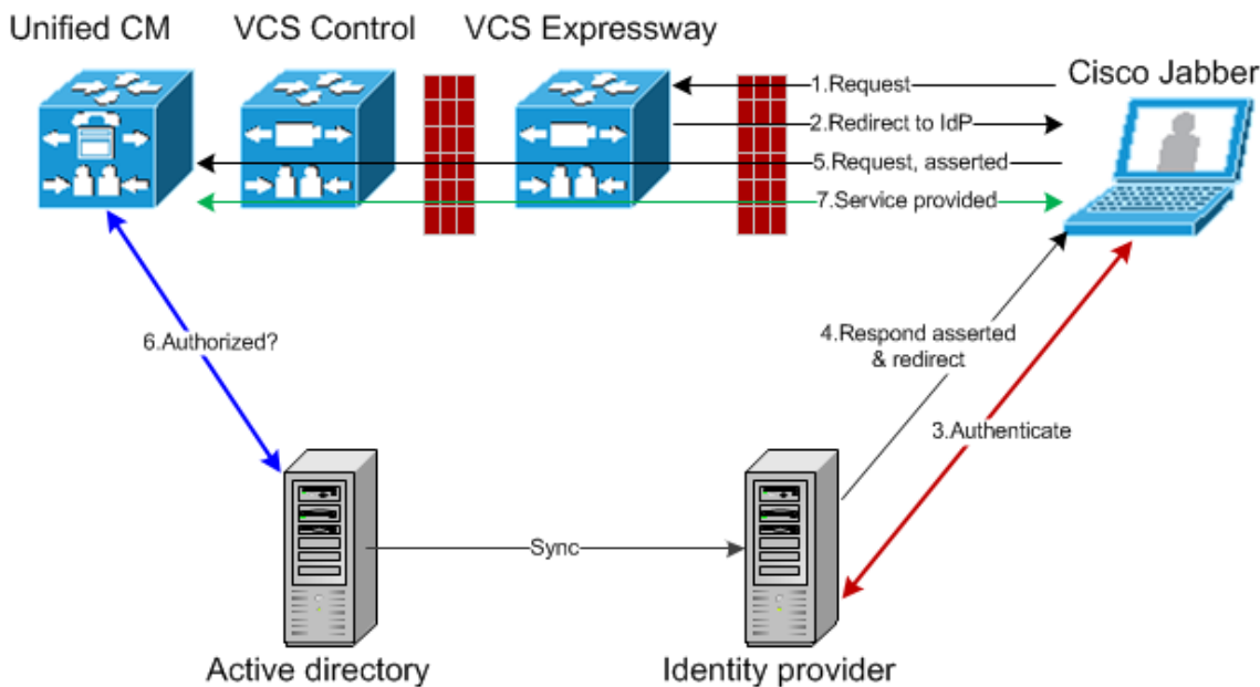
Figure 16 Remote single sign-on for on-premises UC services
