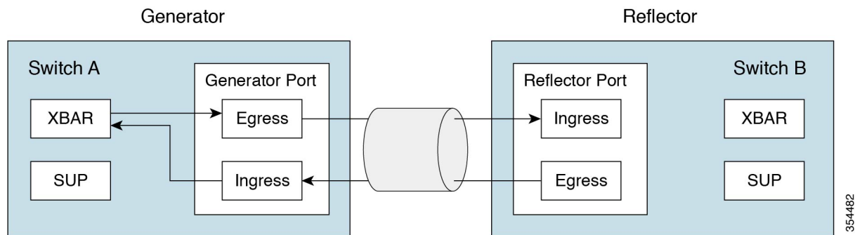
Figure 2: Latency Test
