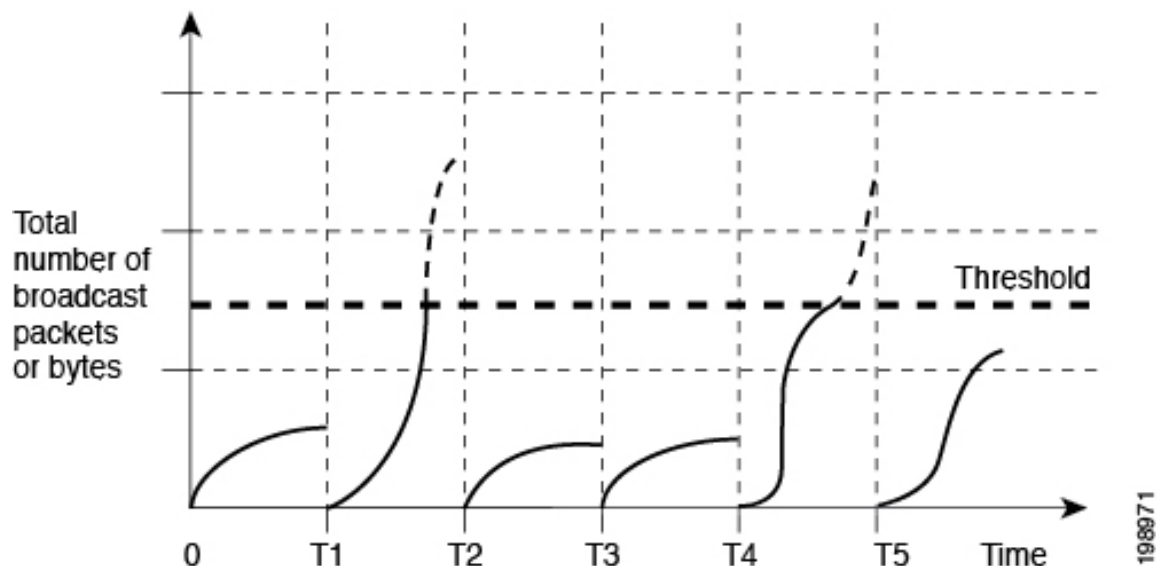
Figure 19: Broadcast Suppression
