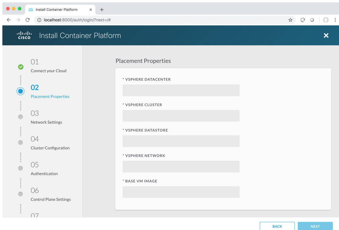
Figure 13: Placement Properties Screen
