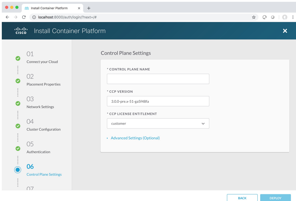
Figure 17: Control Plane Settings Screen
