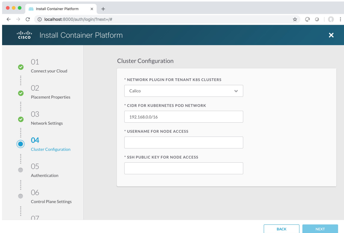
Figure 15: Cluster Configuration Screen
