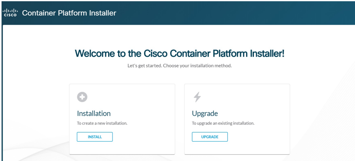
Figure 11: Welcome Screen
