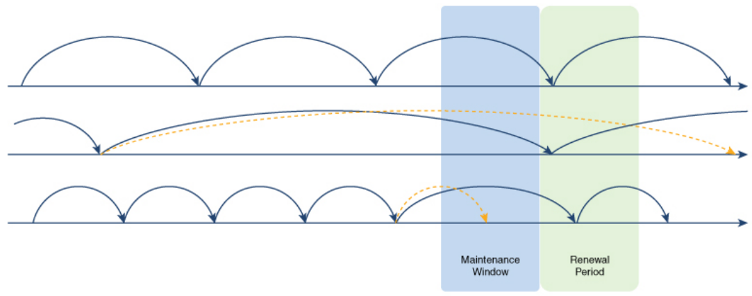
Figure 1: Maintenance Window
