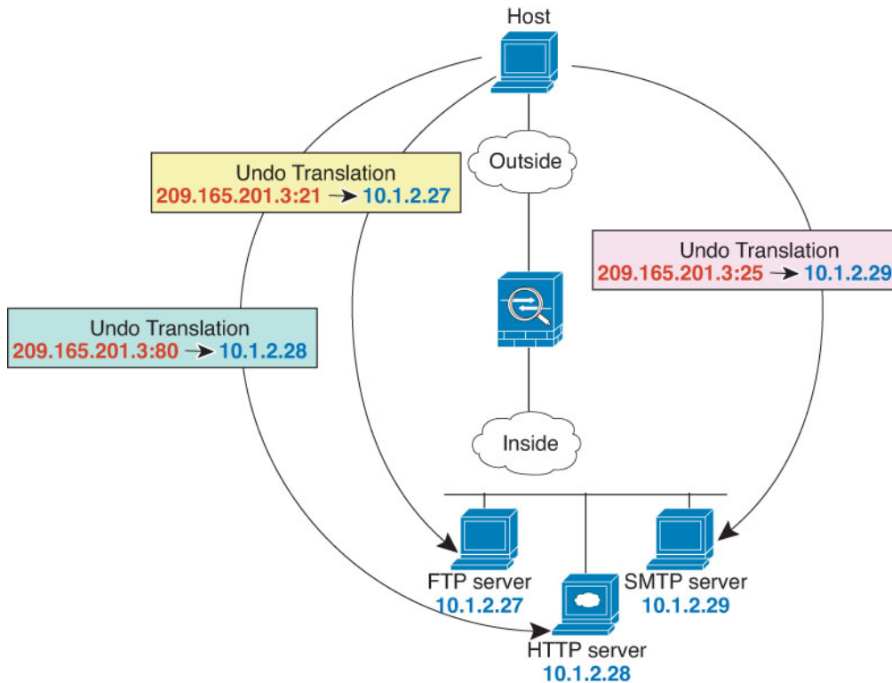
Figure 14: Static NAT-with-Port-Translation
