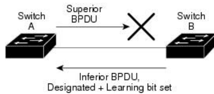
Figure 7: Detecting Unidirectional Link Failure
