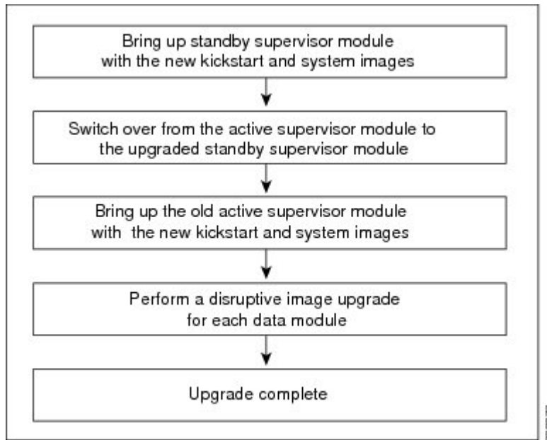
Figure 1: ISSU Process
