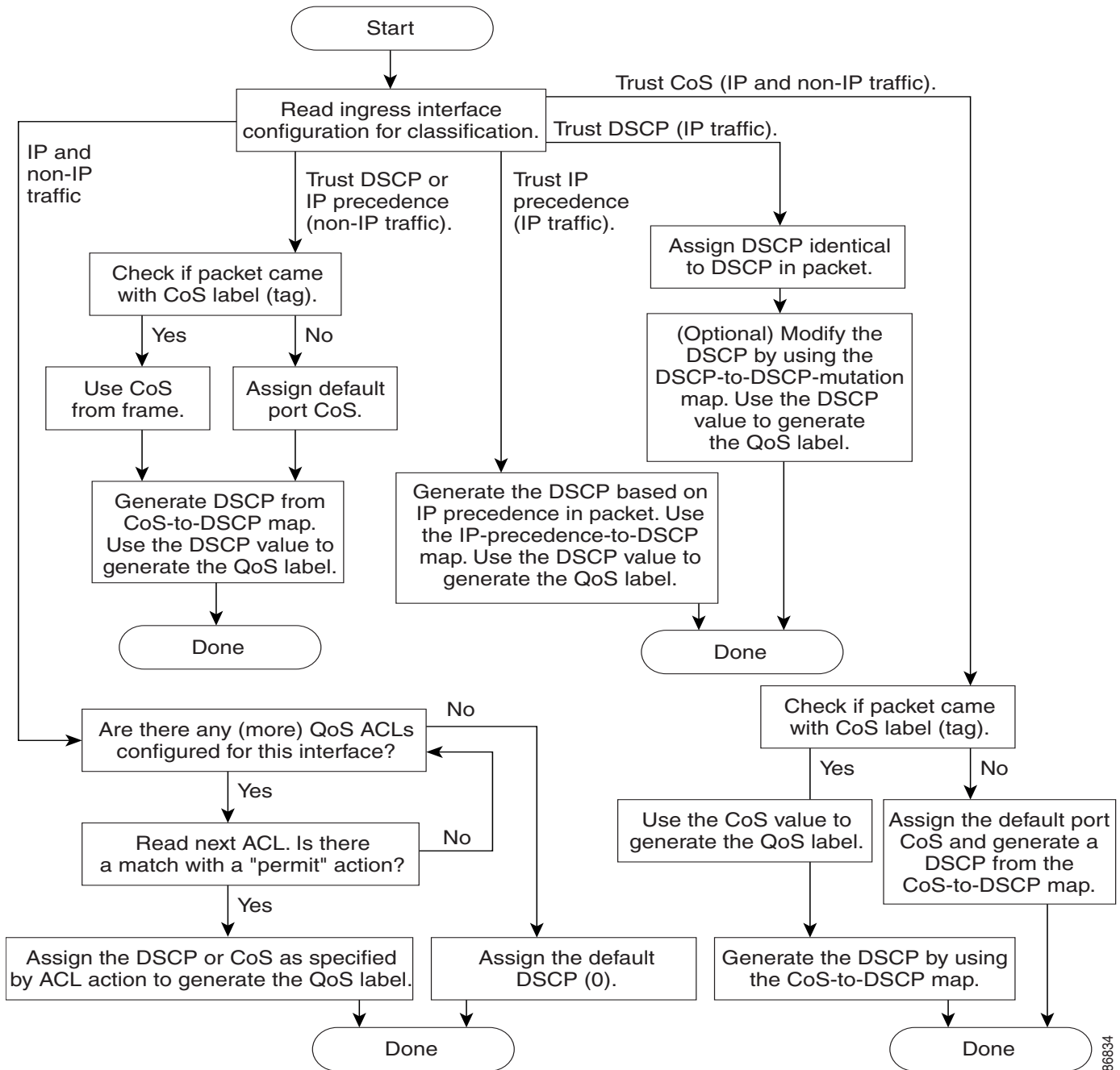
Figure 34-3 Classification Flowchart
