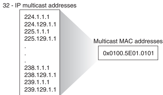
Figure 43-4 MAC Address Ambiguities
