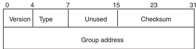
Figure 43-5 IGMP Version 1 Packet Format
