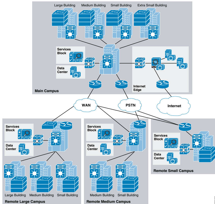
Figure 2 shows the service fabric design model used in the community college LAN design.
