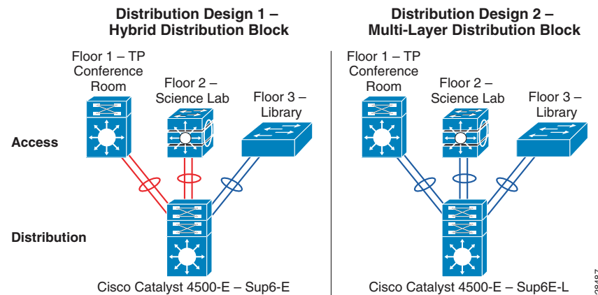
Figure 21 Two Cisco Catalyst 4500-E-Based Distribution Layer Options
