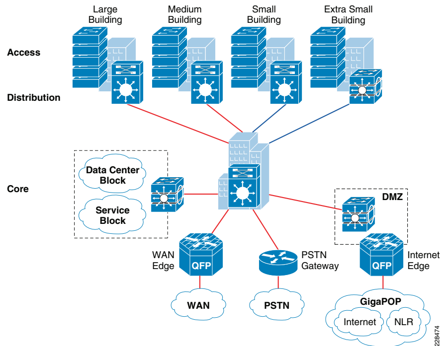
Figure 7 Main College Campus Site Reference Design
