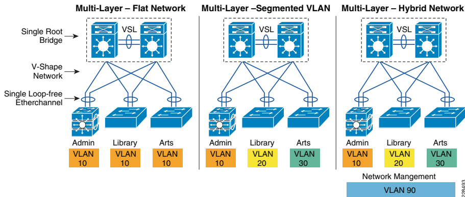
Figure 27 Multilayer Design Variations
