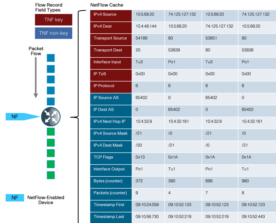
Figure 1 - TNF cache
