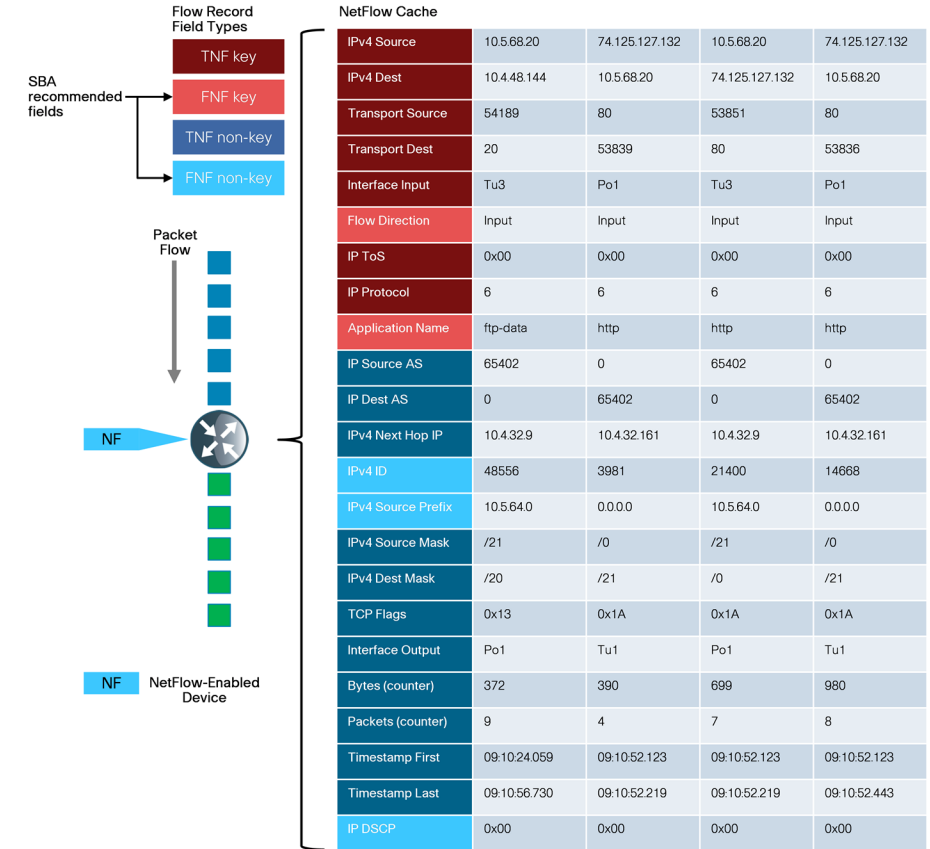
Figure 3 - FNF cache
