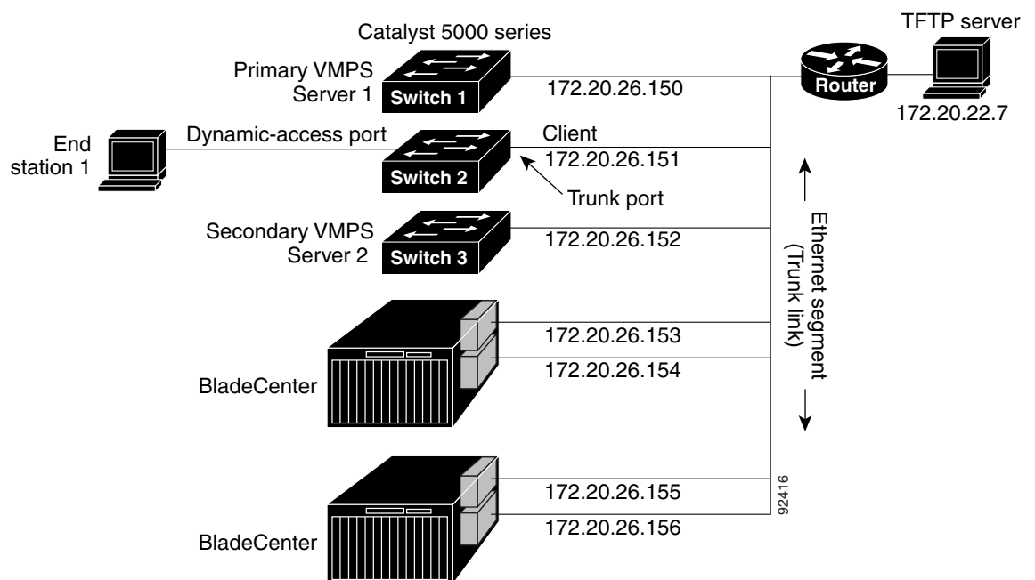
Figure 13-5 Dynamic Port VLAN Membership Configuration
