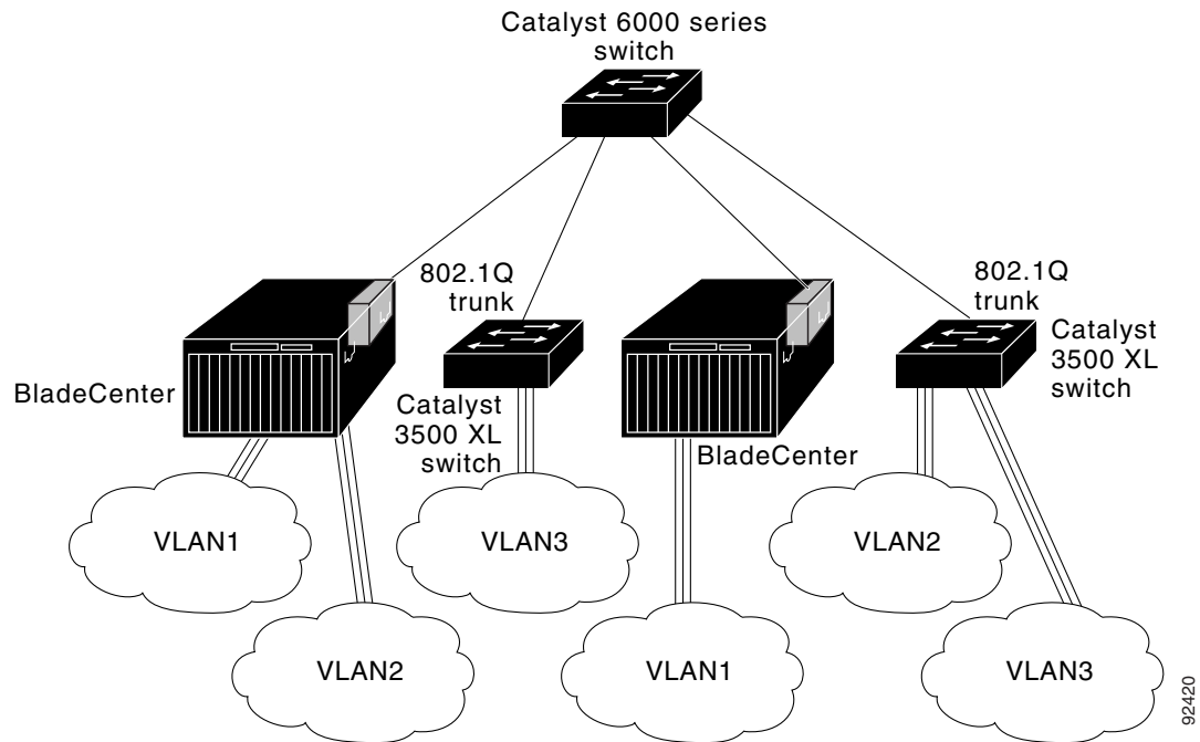
Figure 13-2 Switches in an IEEE 802.1Q Trunking Environment
