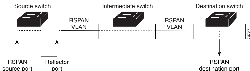
Figure 19-2 Example of RSPAN Configuration
