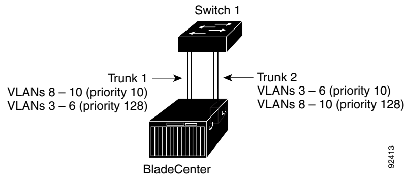
Figure 13-3 Load Sharing by Using STP Port Priorities
