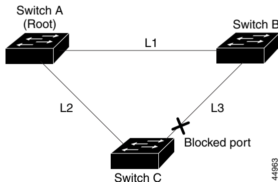
Figure 12-5 BackboneFast Example Before Indirect Link Failure
