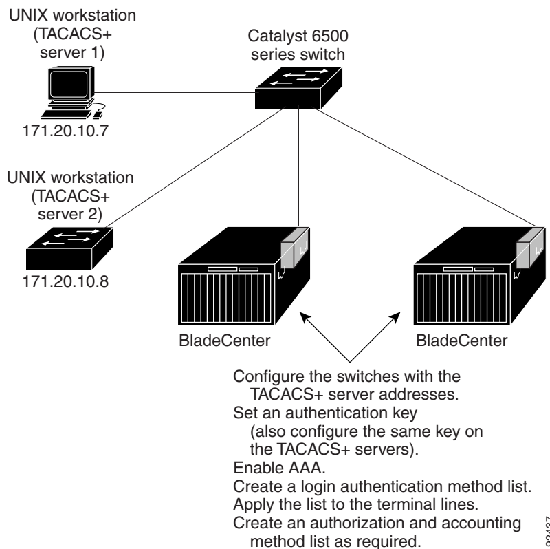
Figure 6-1 Typical TACACS+ Network Configuration
