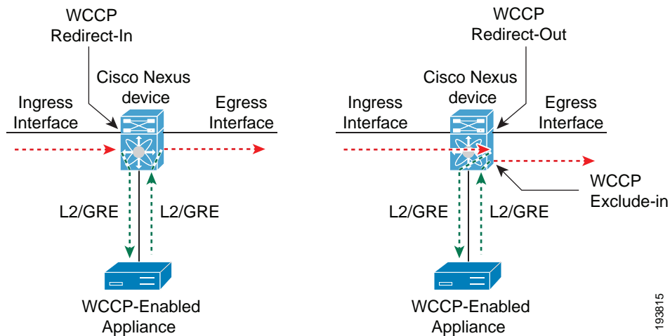
Figure 5-2 WCCP Redirection
