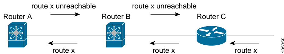
Figure 12-1 RIP with Split Horizon Poison Reverse
