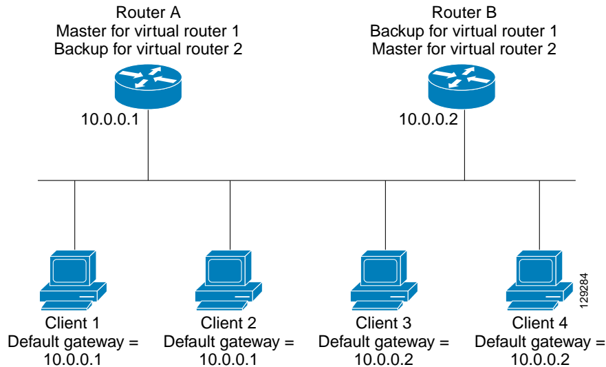
Figure 20-2 Load Sharing and Redundancy VRRP Topology
