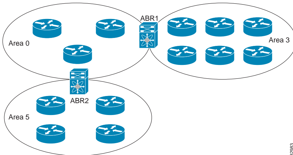
Figure 6-2 OSPFv2 Areas
