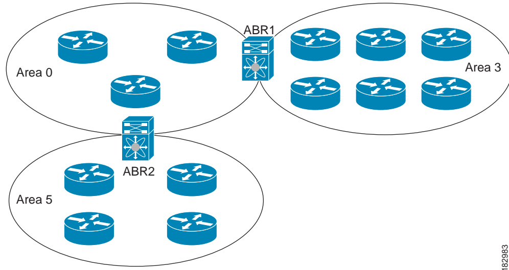
Figure 7-2 OSPFv3 Areas
