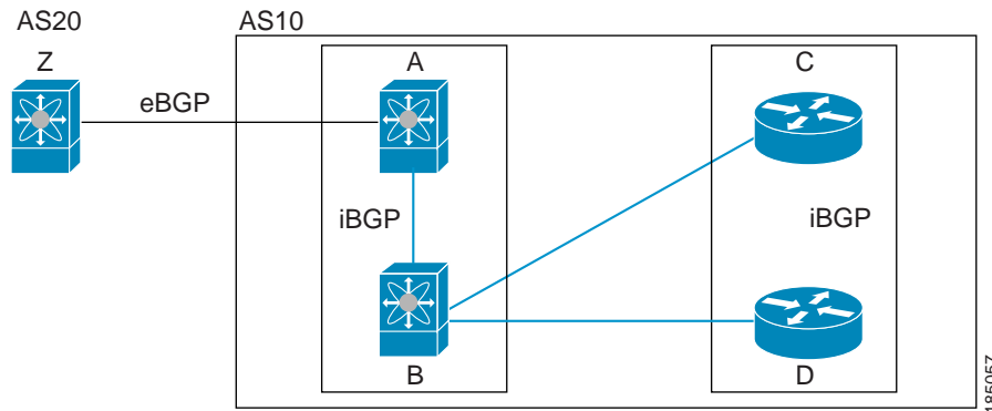
Figure 11-3 Route Reflector
