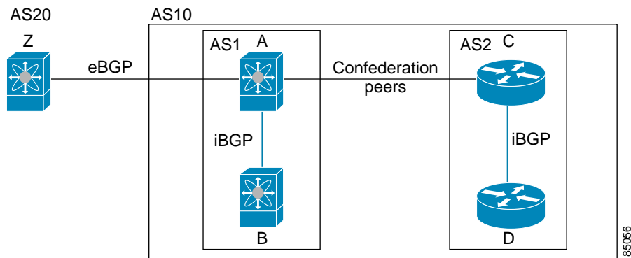
Figure 11-2 AS Confederation
