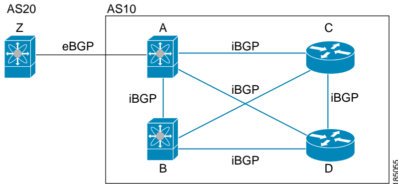
Figure 11-1 iBGP Network
