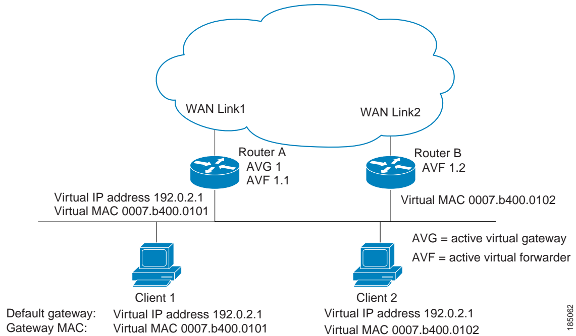
Figure 18-1 GLBP Topology
