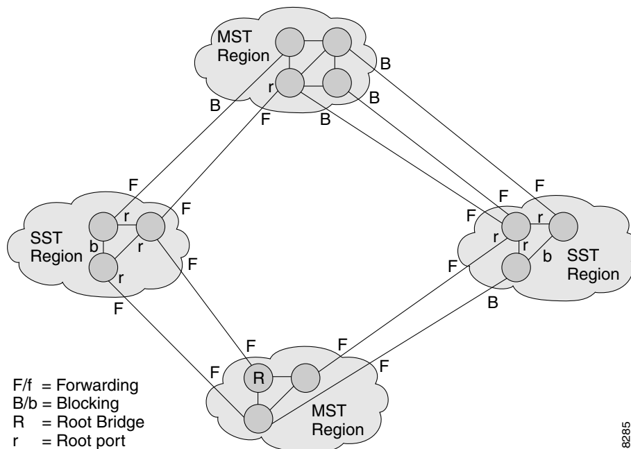
Figure 14-1 Network with Interconnected SST and MST Regions
