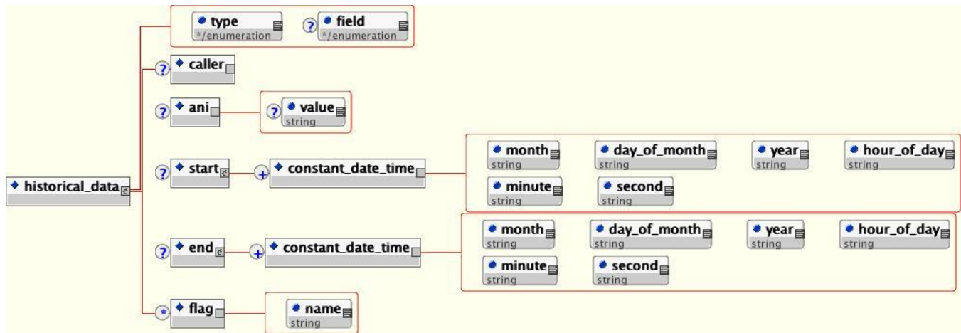
Figure 18: historical data Tag
