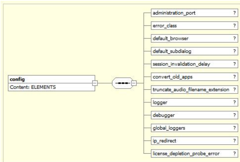
Figure 23: Global Configuration Options
