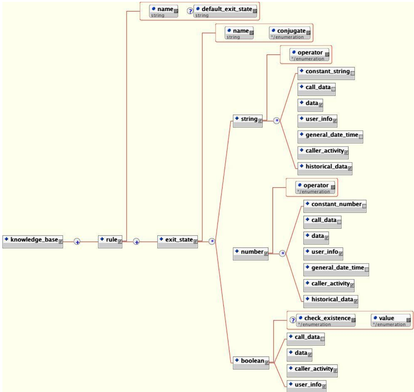
Figure 12: Example of Tags for Defining a Decision
