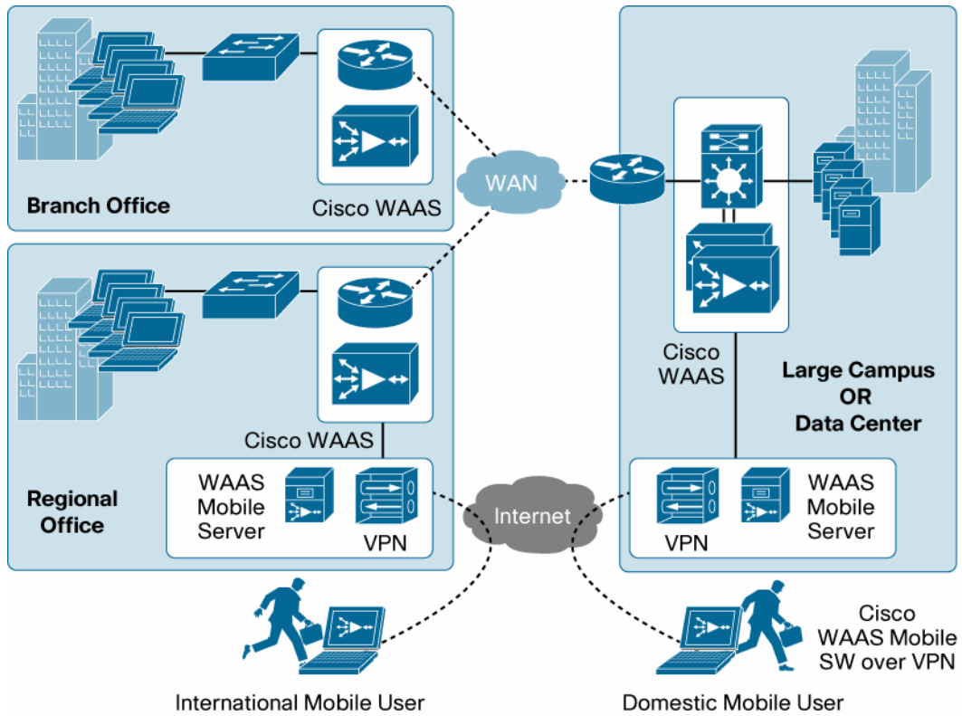
Figure 3. Cisco WAAS Mobile Extends Cisco WAAS Deployment
