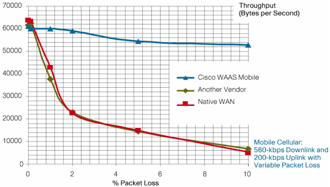
Figure 1. Industry-leading Application Throughput Improvement
