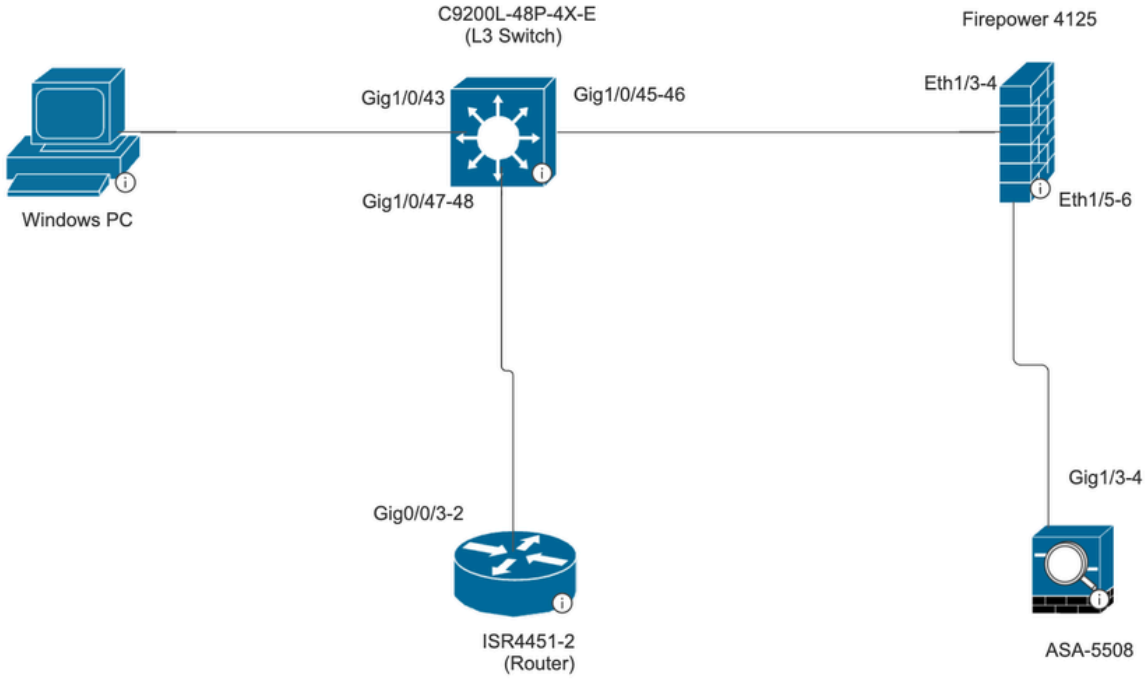
Figure 1. Topology
