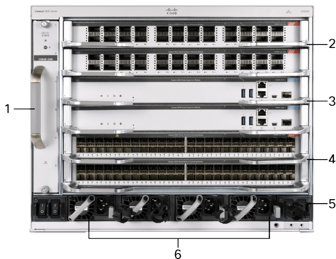
Figure 1. Front view of a Cisco Catalyst 9606R
