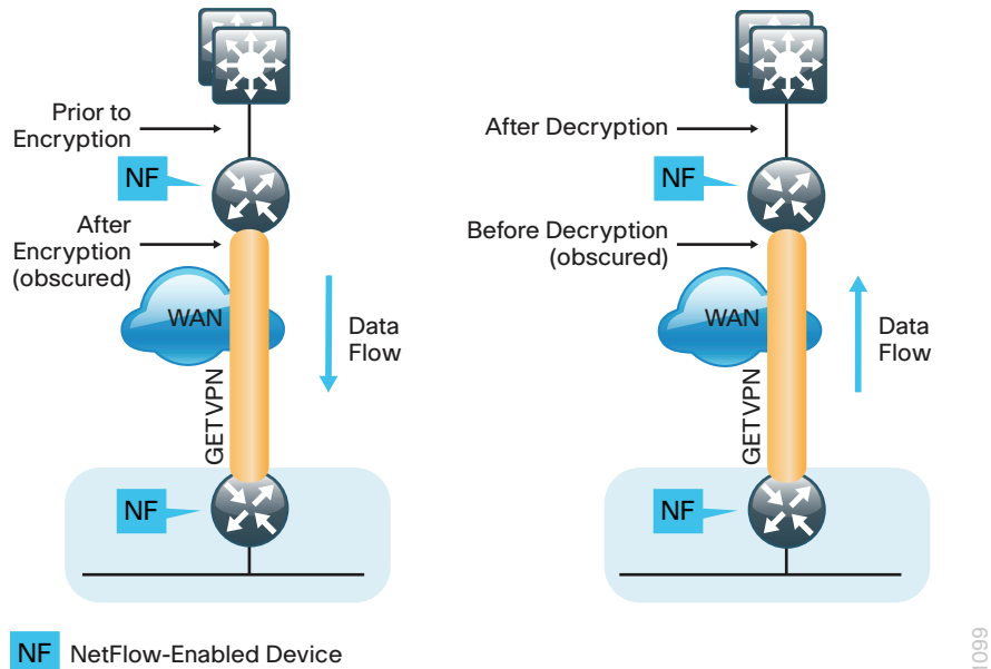
Figure 4 - Encryption and NetFlow
