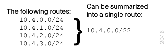
Figure 2 - Route summarization
