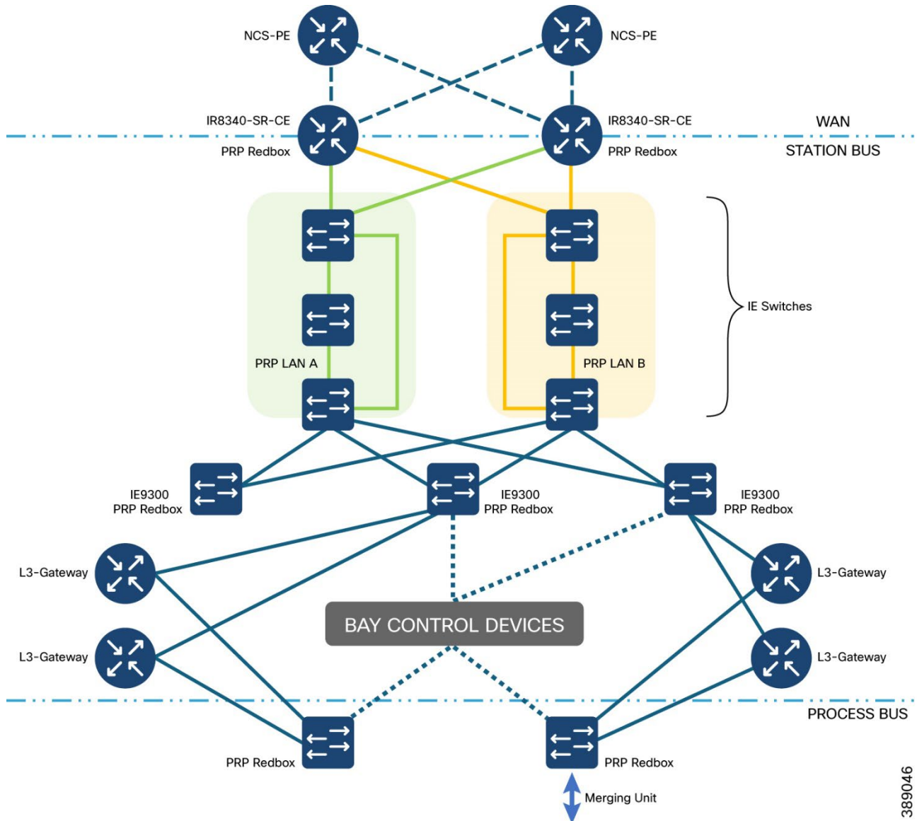
Figure 13 PRP for Station bus and Process bus
