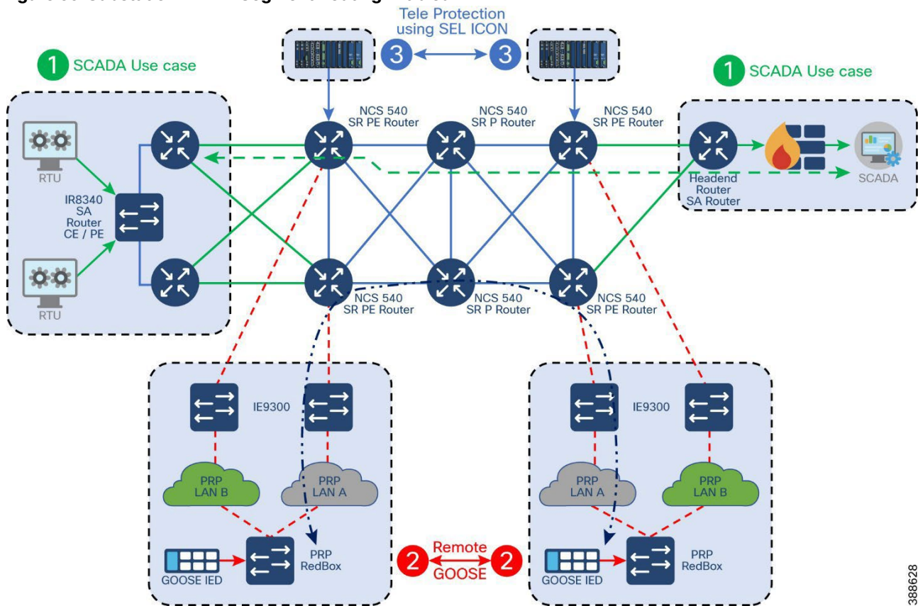
Figure 35 Substation WAN - Segment Routing Enabled
