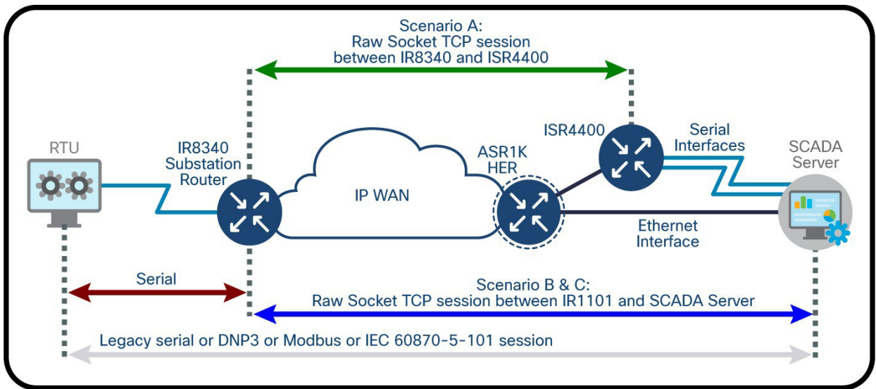
Figure 28 Raw Socket TCP Transport
