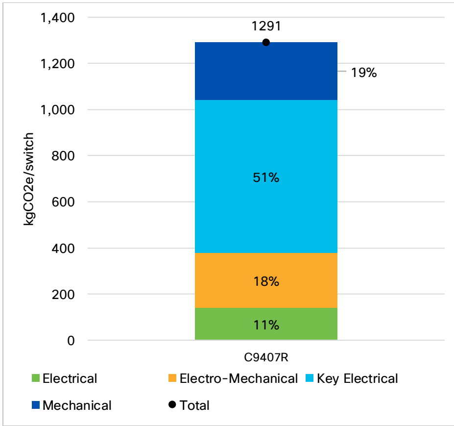
Figure 4: Global Warming Potential per C9407R from Manufacturing Components Across the Upstream Supply Chain
