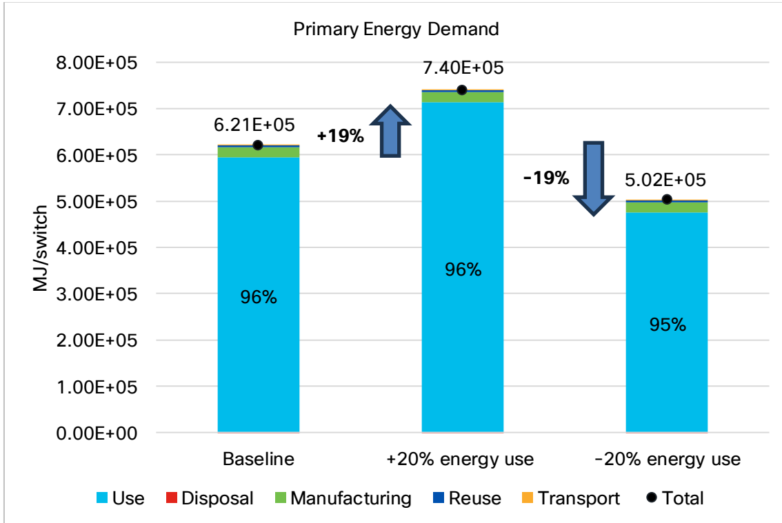
Figure 12: Primary Energy Demand Sensitivity Analysis for Change in Energy Use
