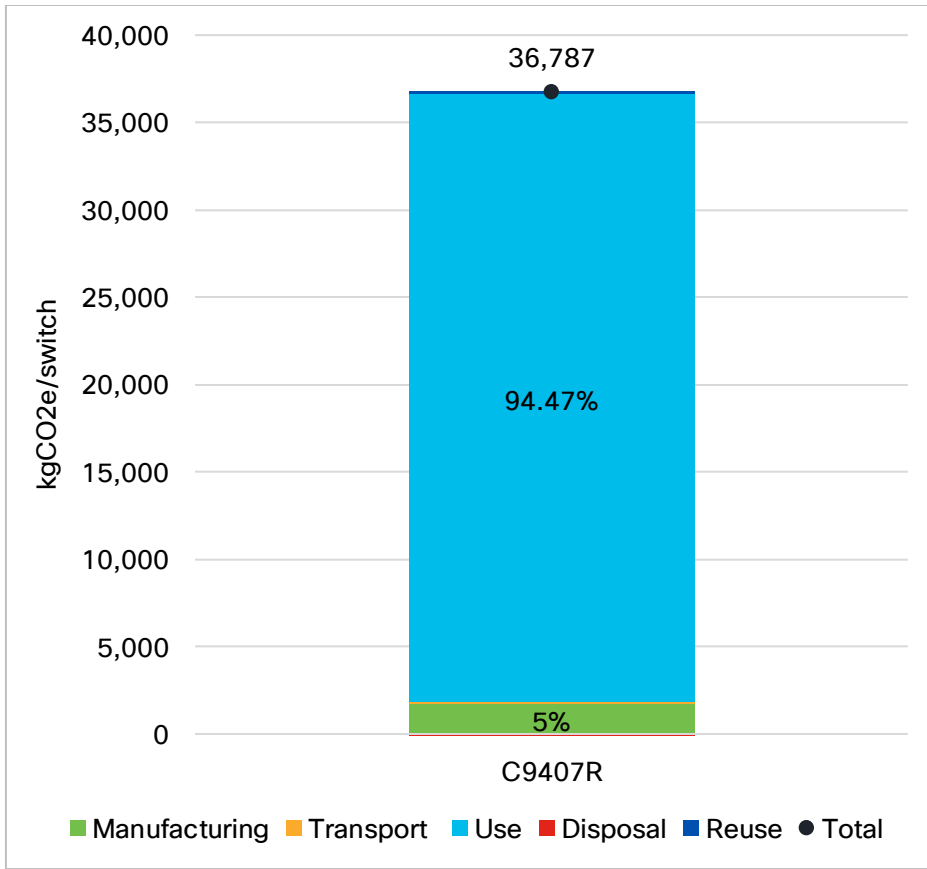
Figure 3: Global Warming Potential per C9407R by Life Cycle Stage
