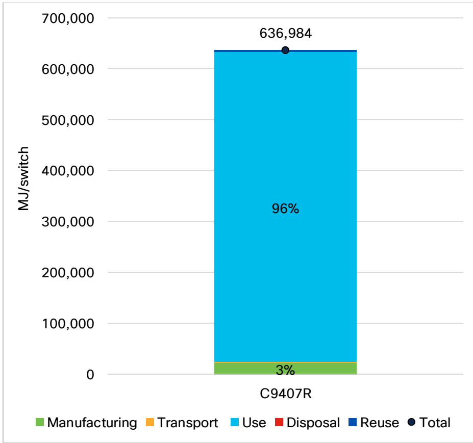
Figure 5: Primary Energy Demand per 9407R by Life Cycle Stage
