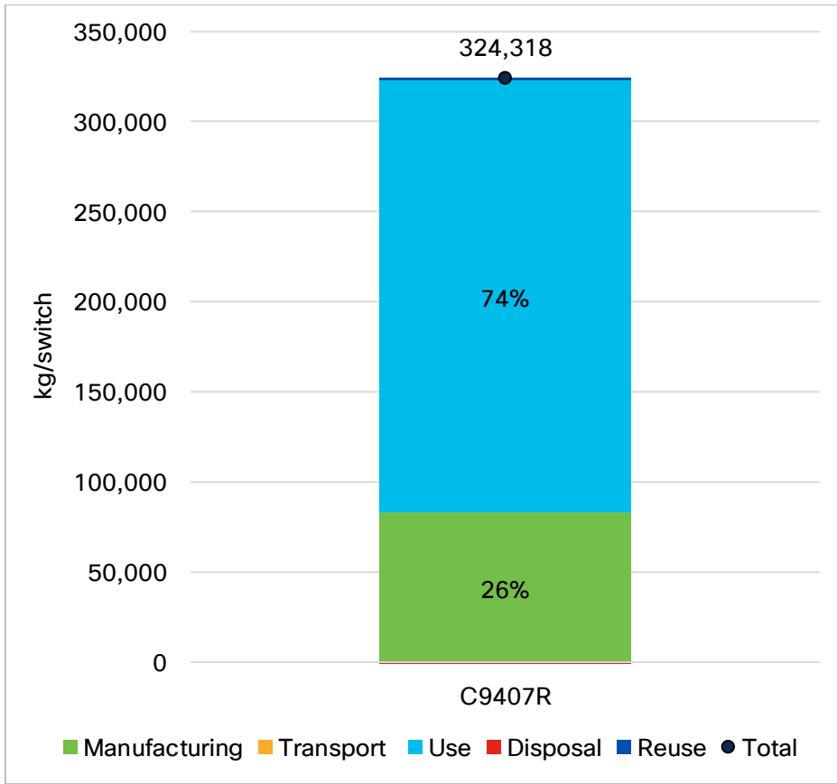
Figure 6: Blue Water Consumption per 9407R by Life Cycle Stage
