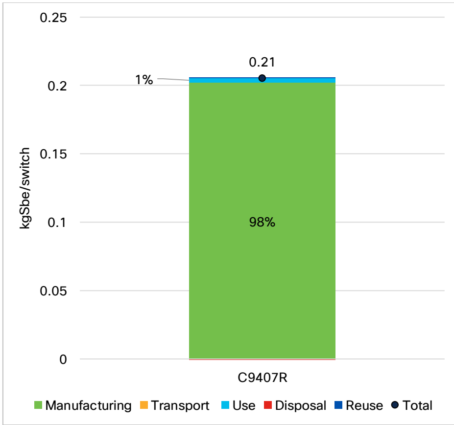
Figure 7: Abiotic Depletion Potential per C9407R by Life Cycle Stage
