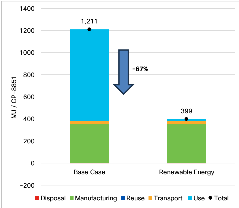
Figure 12: Sensitivity Analysis Results for Primary Energy Demand with Renewable Energy Sourcing
