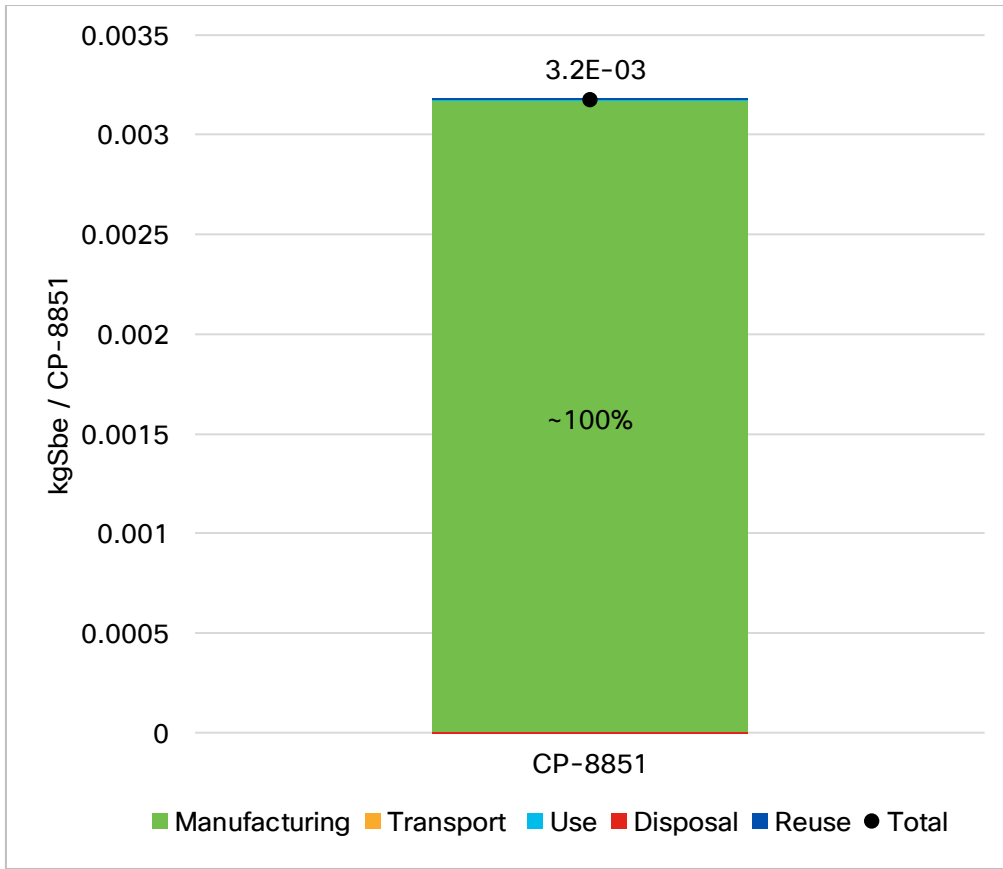
Figure 7: Abiotic Depletion Potential of CP-8851 by Life Cycle Stage
