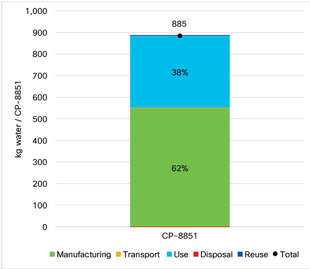
Figure 6: Blue water Consumption of CP-8851 by Life Cycle Stage
