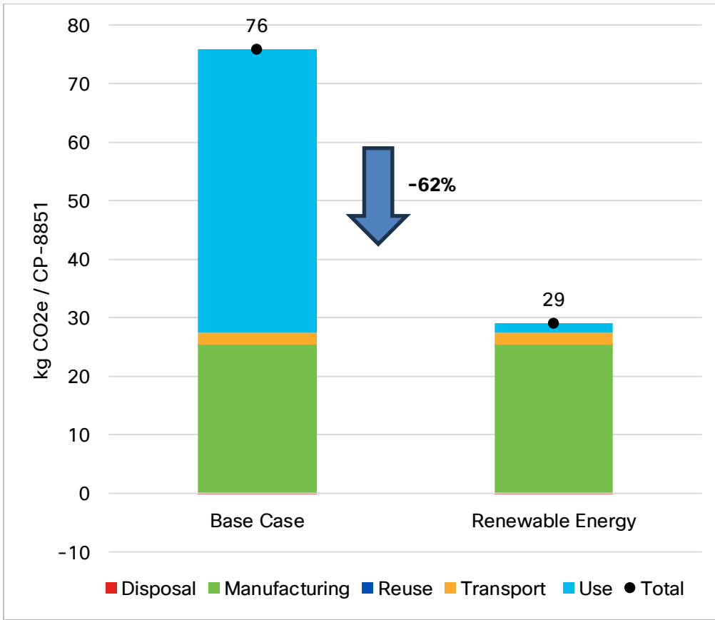
Figure 11: Sensitivity Analysis Results for GHG Emissions with Renewable Energy Sourcing
