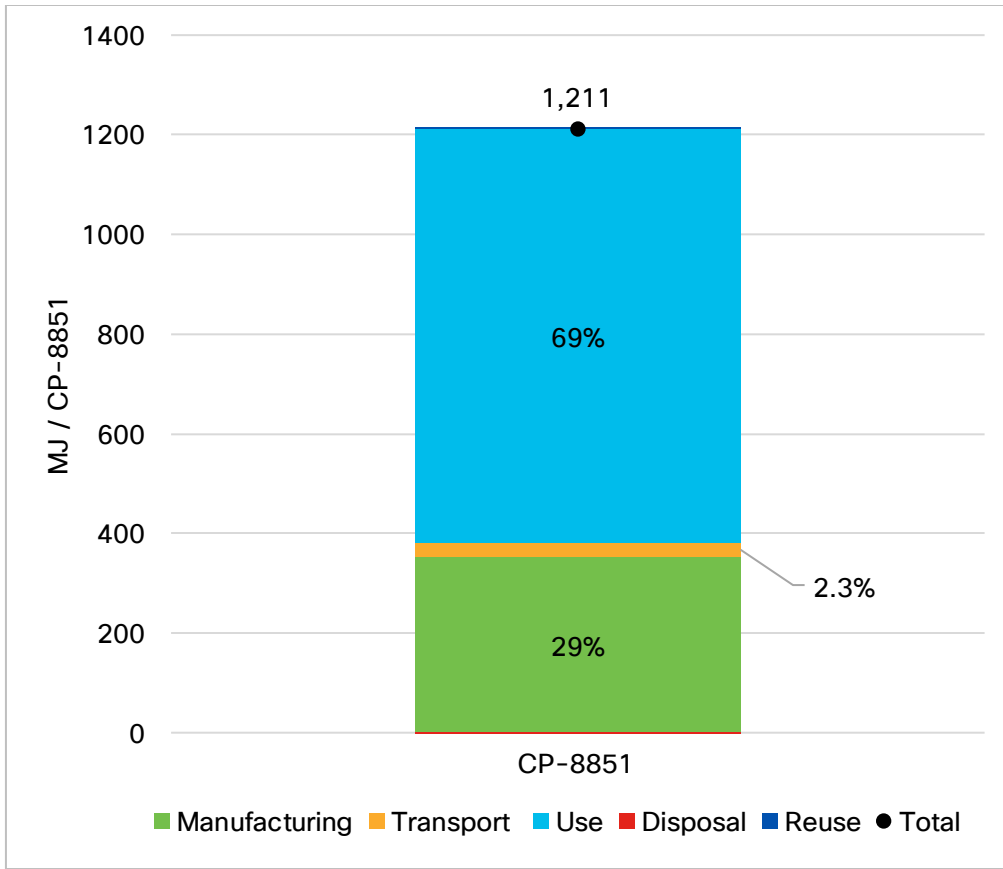
Figure 5: Primary Energy Demand of CP-8851 by Life Cycle Stage
