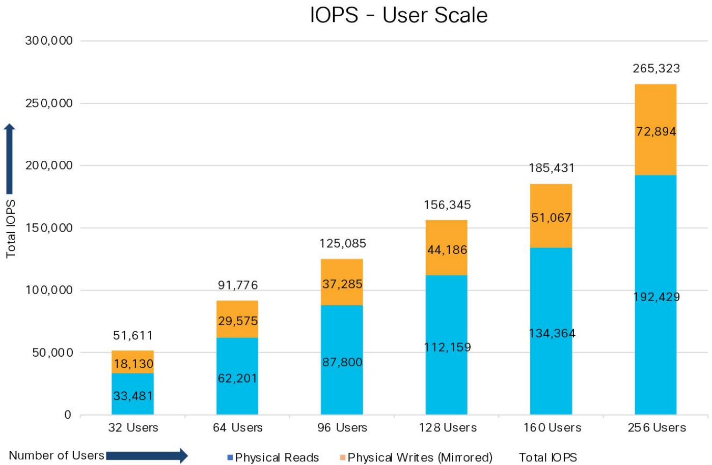
Figure 13. IPOS for CDBDB database for different numbers of users
