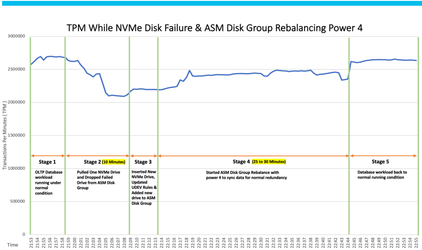
Figure 15. Summary of TPM for failure test
