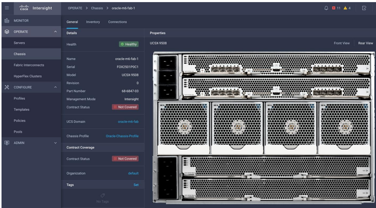
Cisco UCS X9508 Server chassis (rear view)
