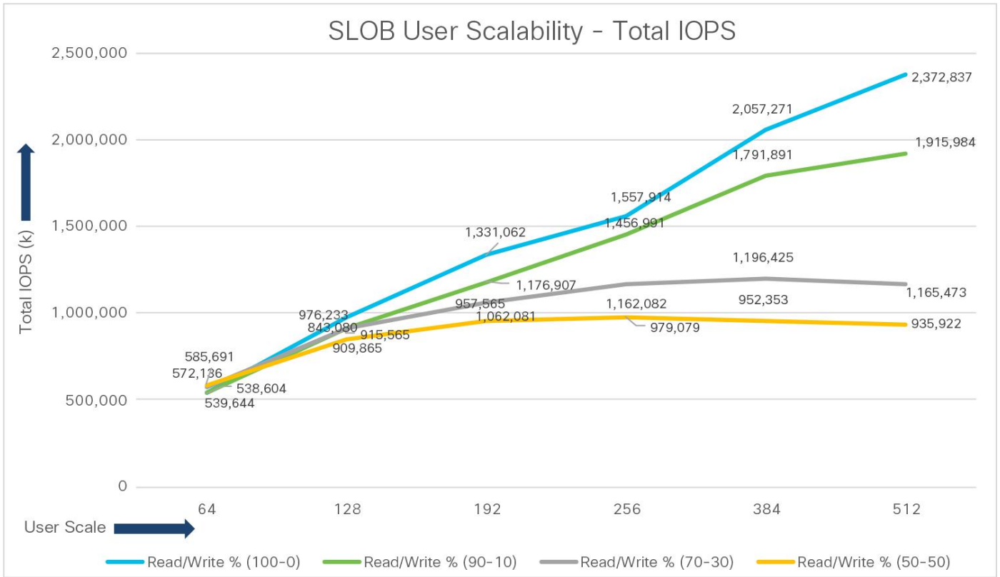
Figure 11. Total number of IOPS for test scenarios
