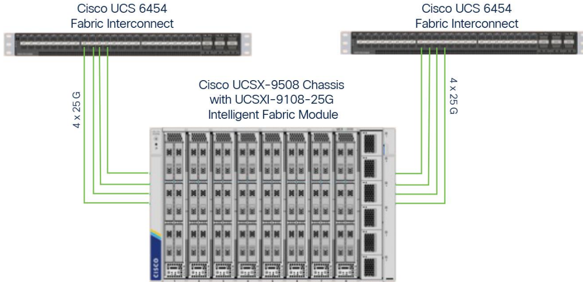
Figure 1. Sample configuration of Cisco UCS X9508 chassis connected to each Cisco UCS 6454
