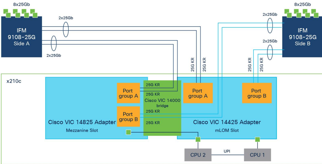
Figure 7. Cisco VIC 14425 and 14825 in Cisco UCS X210c M6
