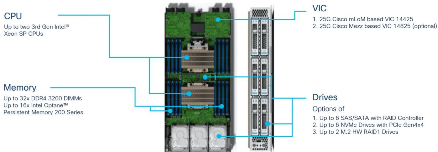
Figure 5. Cisco UCS X210c M6 Compute Node
