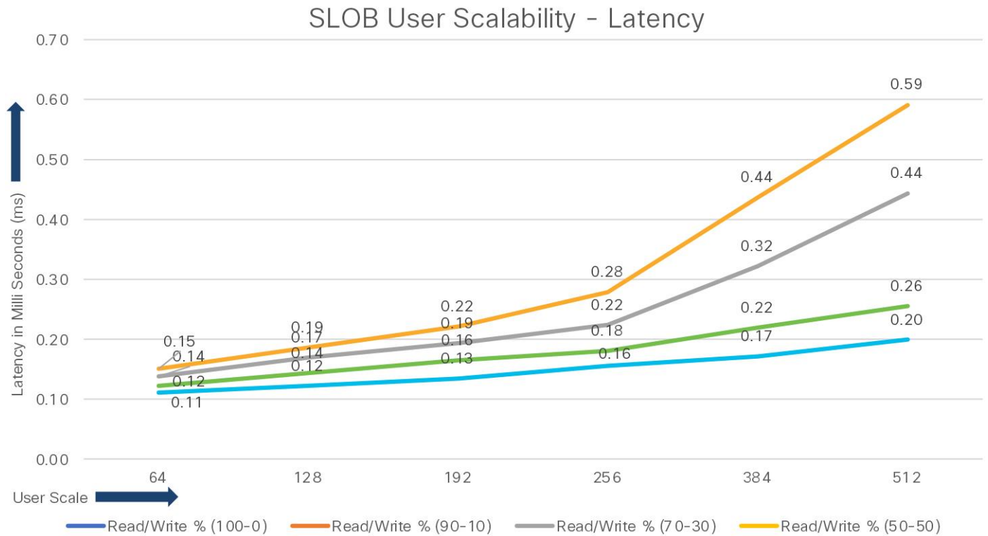
Figure 12. Latency by local storage across different workloads
