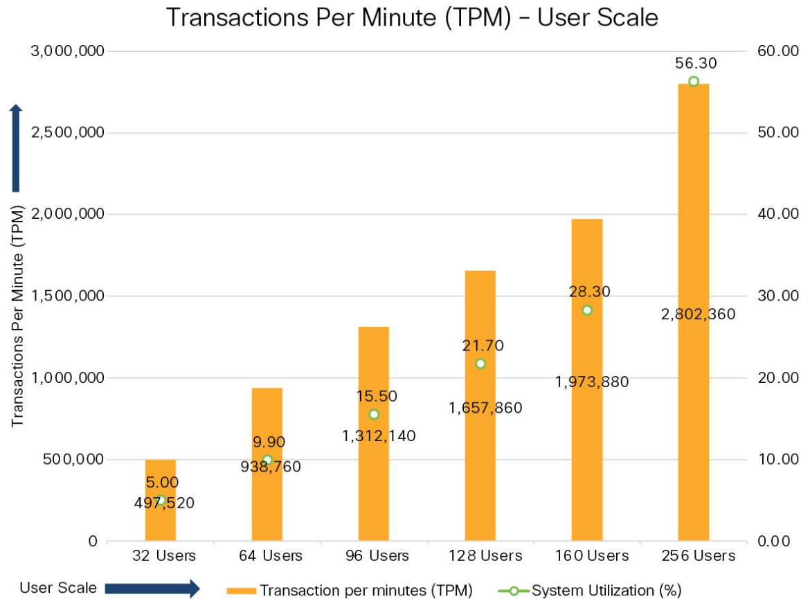
Figure 14. RPM and system usage for tests in Table 3
