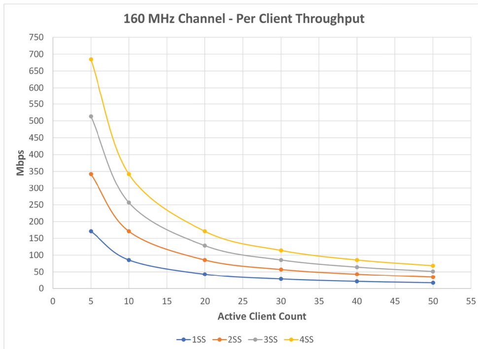
Figure 2: Throughput for different number of spatial streams for increasing numbers of active client counts. While the maximum throughputs are significantly higher with Wi-Fi 6E, they are still far below wired connections.
