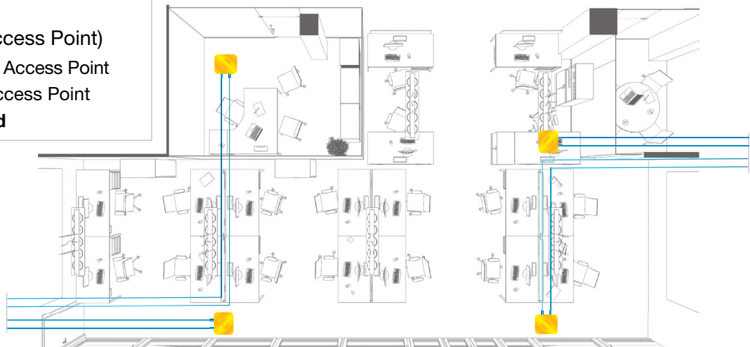
Figure 3: Example of four cables per access point being used to support spectrum partitioning (Day 2) and to support port aggregation for upgrade access point performance (Day 3), all using the same cabling infrastructure installed on Day 1.
