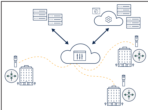
Figure 3. Lossless recovery
