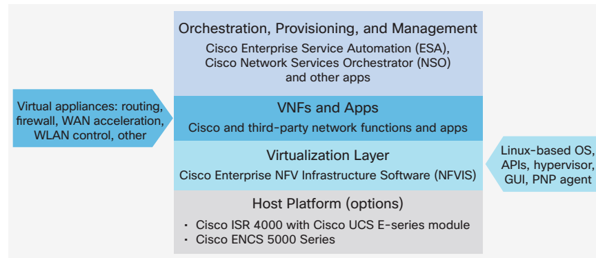
Figure 1. Basic Cisco Enterprise NFV Architecture
