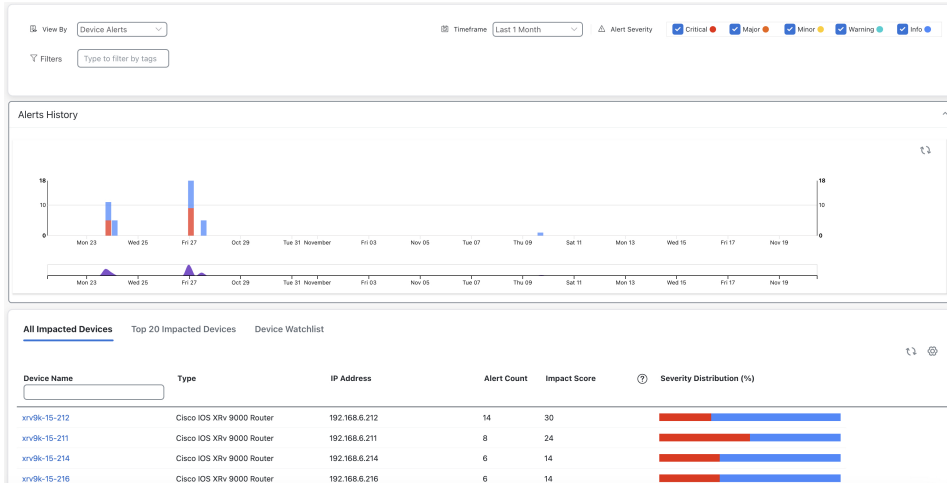
Figure 9: Alert Dashboard
