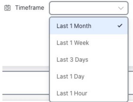
Figure 11: Timeframe Dropdown
