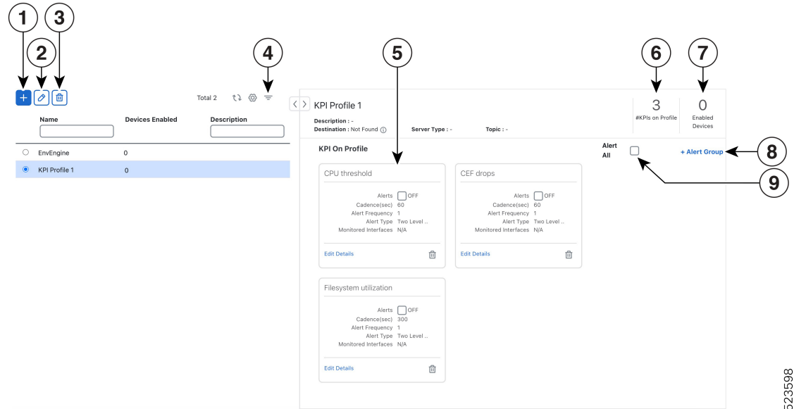
Figure 3: KPI Profiles
