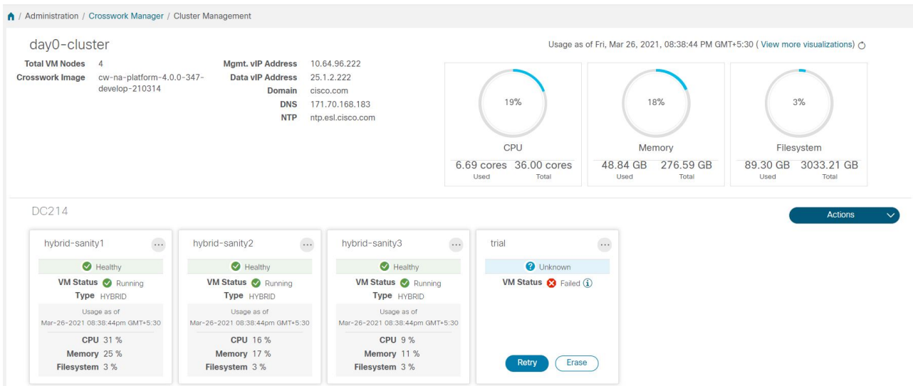
Figure 7: Cluster Management Window: Failed VM Deployment
