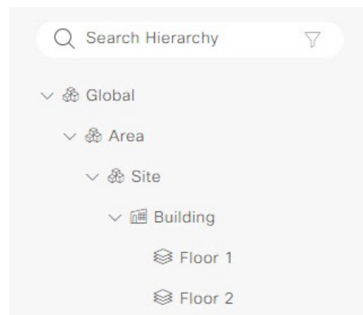
Figure 2: Network Hierarchy
