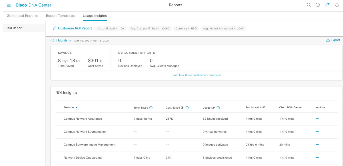
Figure 124: Usage Insights Report Dashboard
