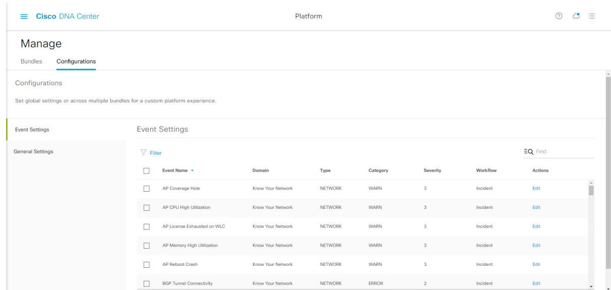
Figure 5: Events Settings Window
