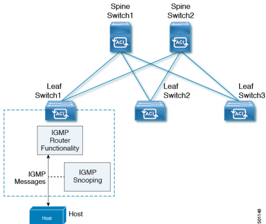
Figure 35: IGMP Snooping function
