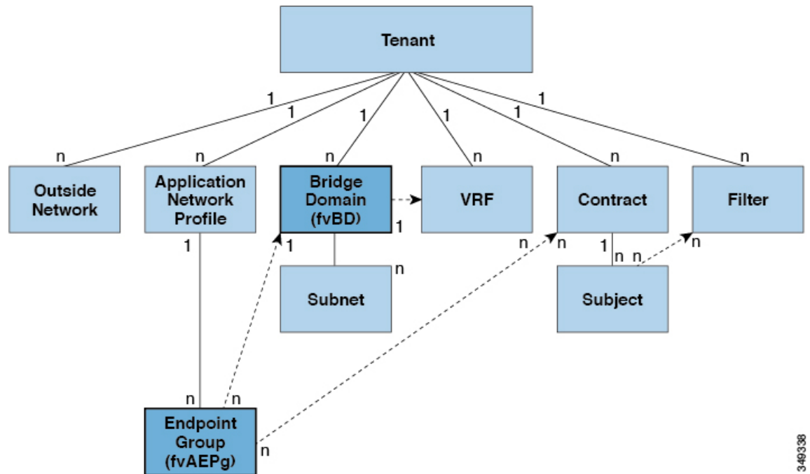
Figure 20: MO Relations
