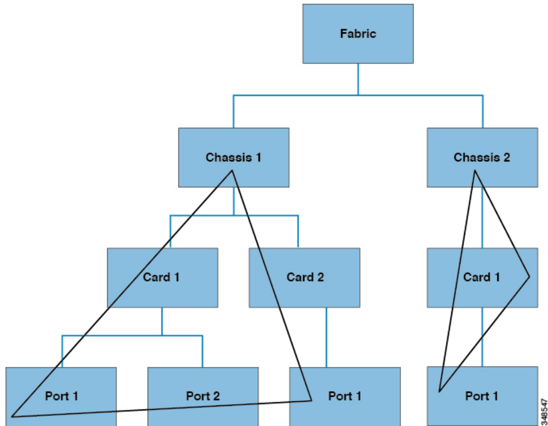
Figure 118: Tree-Level Queries
