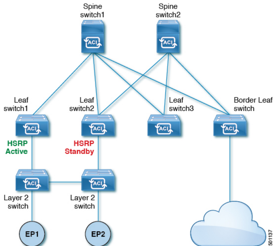
Figure 84: HSRP Deployment Topology
