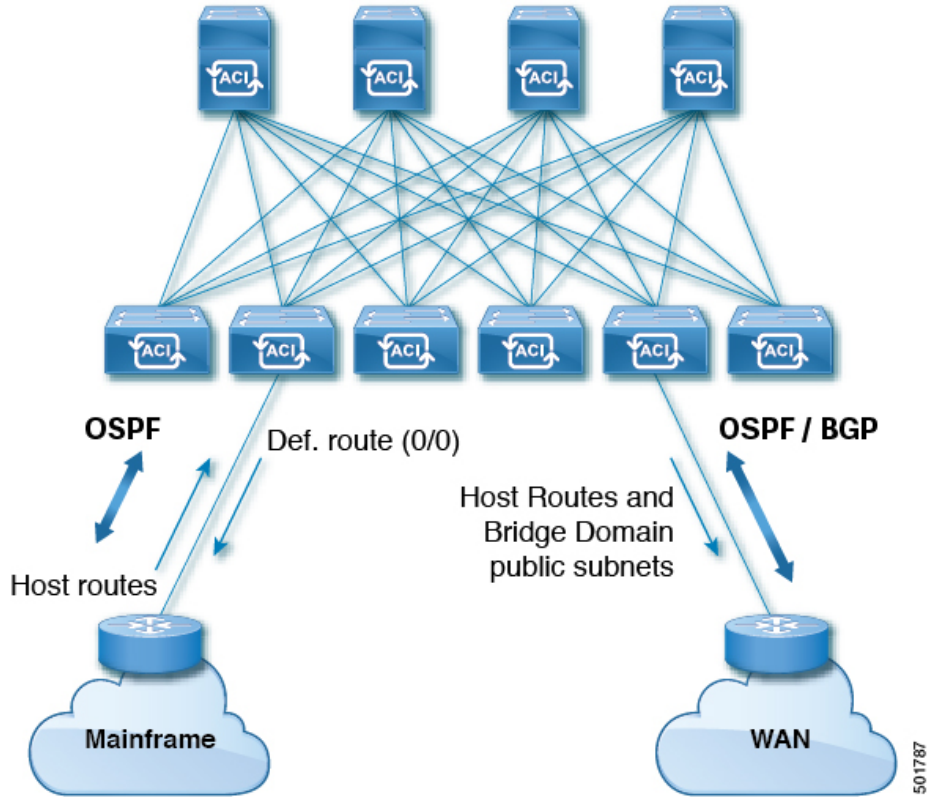
Figure 44: Mainframe Transit Connectivity
