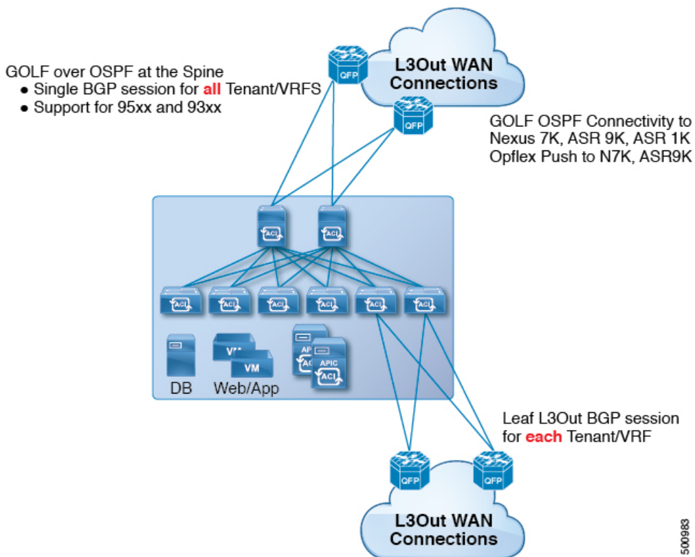
Figure 60: Cisco ACI GOLF Topology
