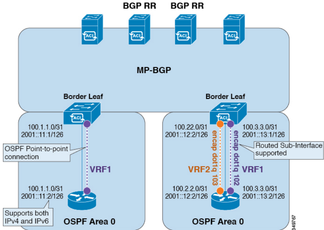
Figure 40: OSPF Layer3 Out Connections
