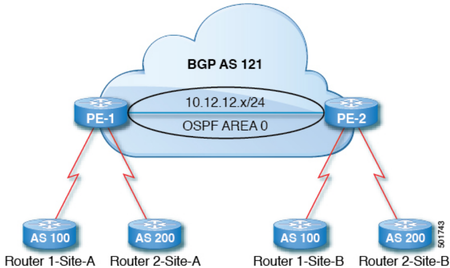
Figure 38: Example Topology Illustrating the Autonomous System Override Process
