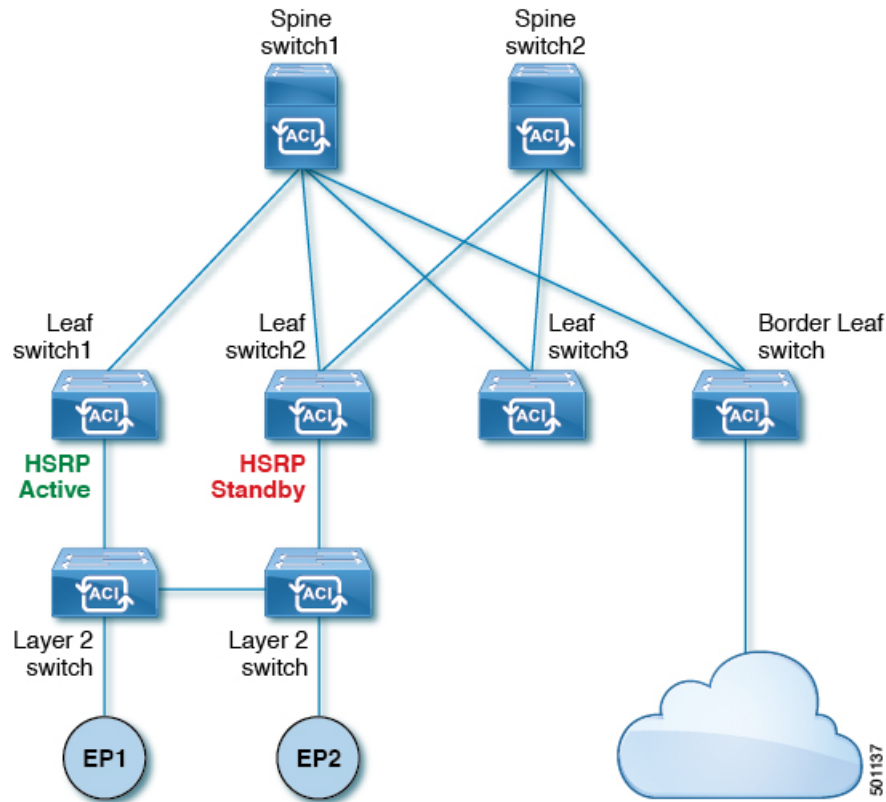
Figure 59: HSRP Deployment Topology
