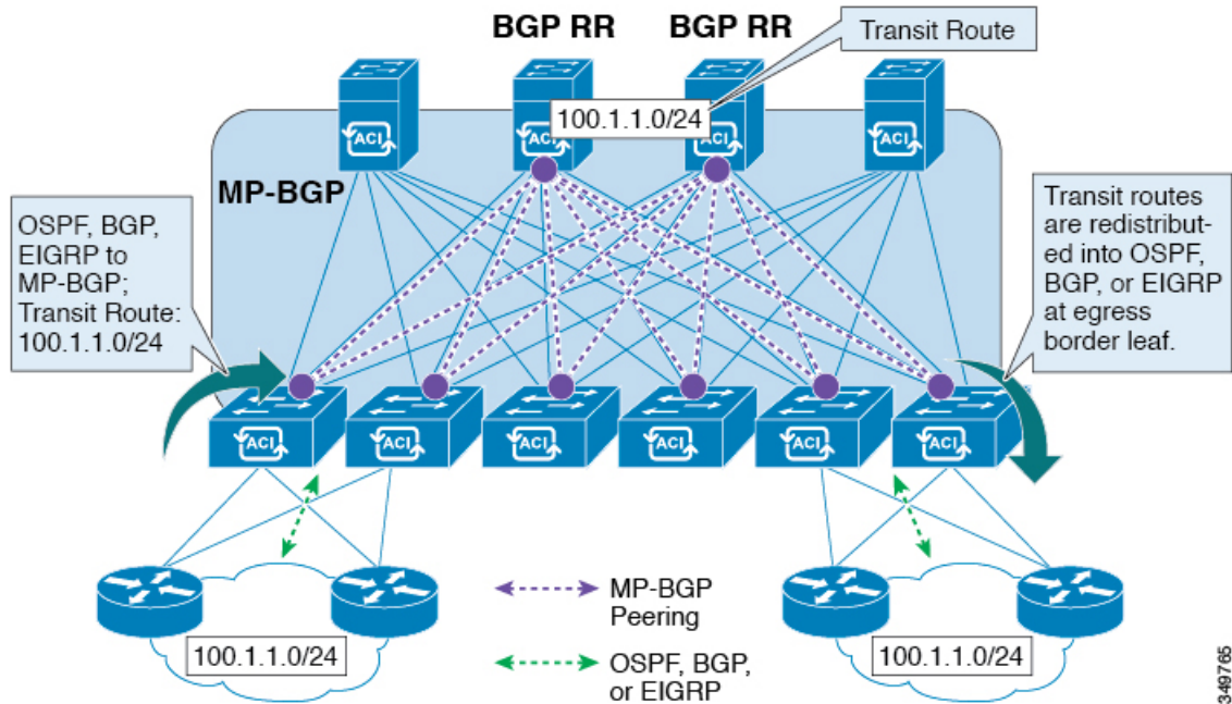
Figure 42: Transit Routing in the Fabric
