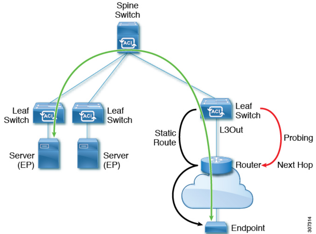
Figure 57: Example ACI L3Out IP SLA
