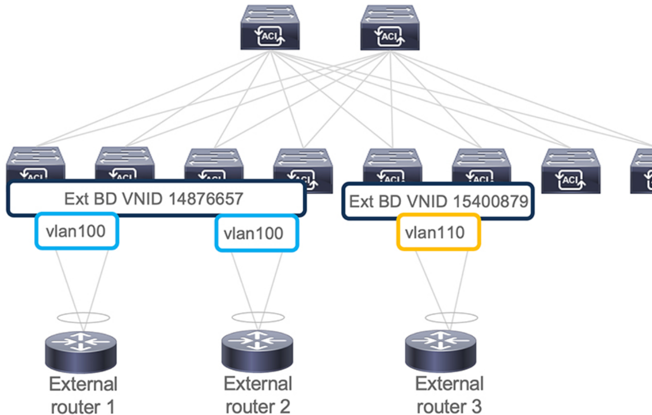
Figure 36: Separate VNID Associated to External Bridge Domains with Different Encapsulation (pre-ACI 5.2(3) Releases).
