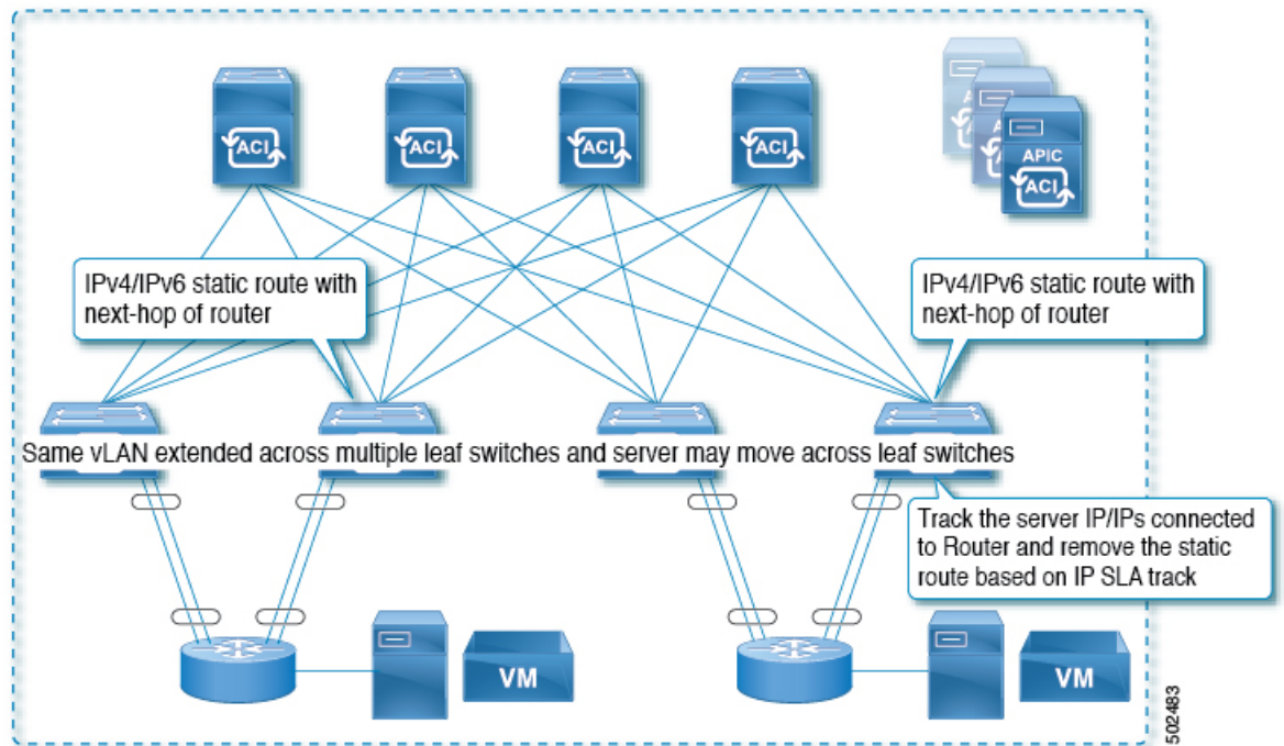
Figure 53: Static Route Removal by Tracking an IP Address Through L3Out
