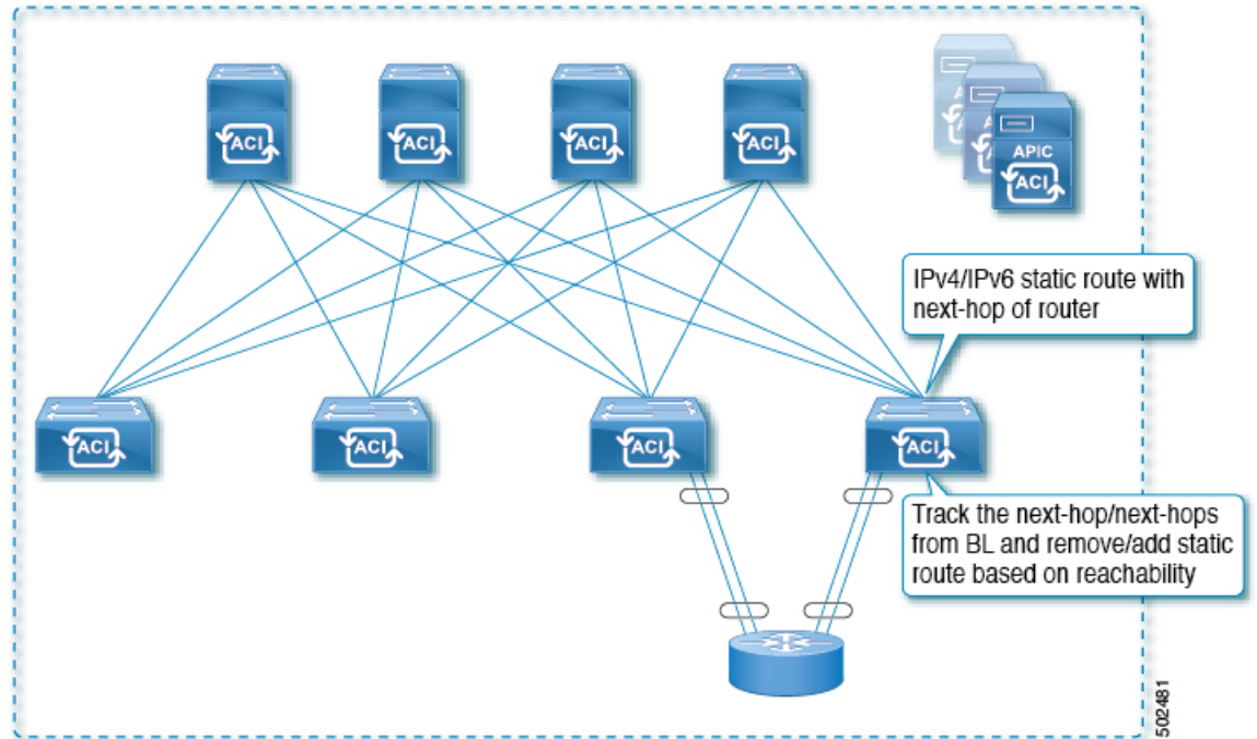
Figure 51: Static Route Availability by Tracking the Next-Hop
