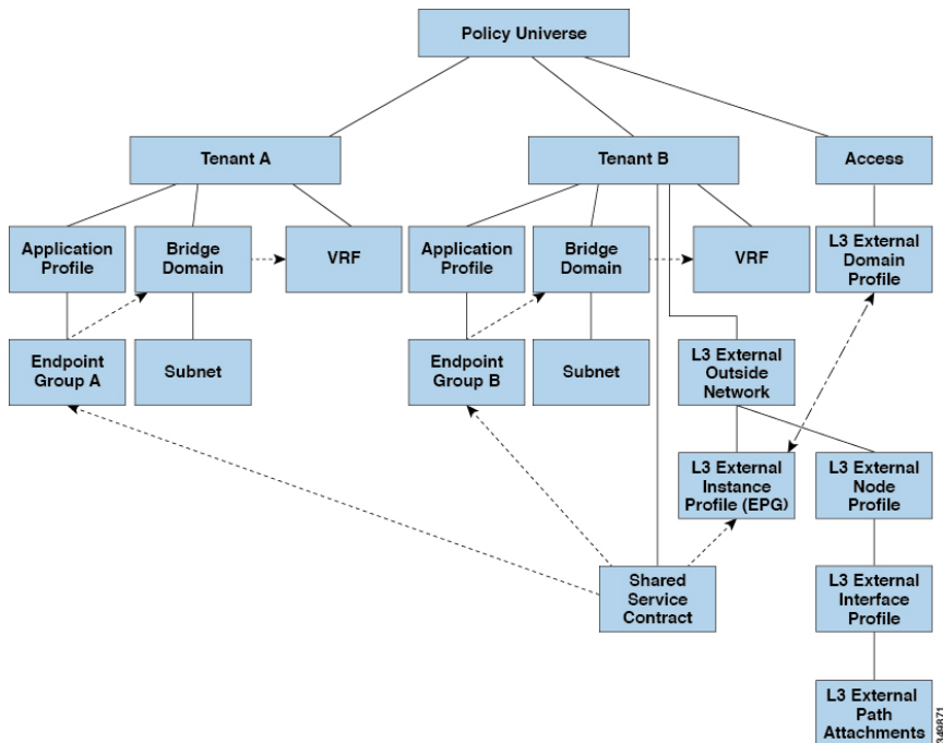
Figure 49: Shared L3Out Policy Model
