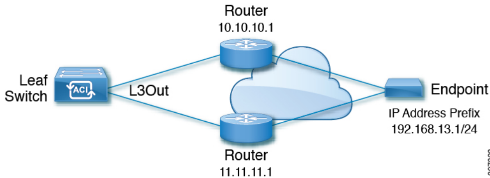
Figure 58: Example Static Route
