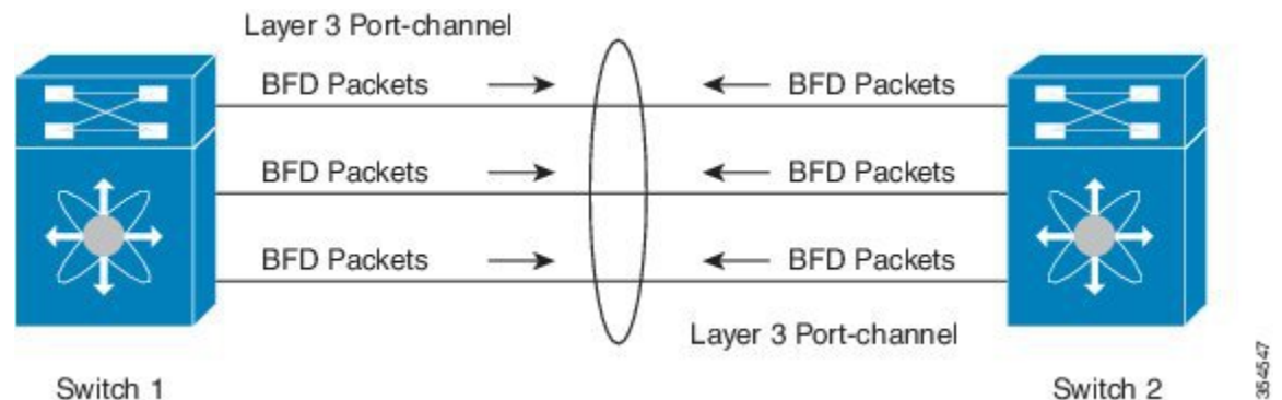
Figure 39: Micro BFD Sessions on a Port Channel
