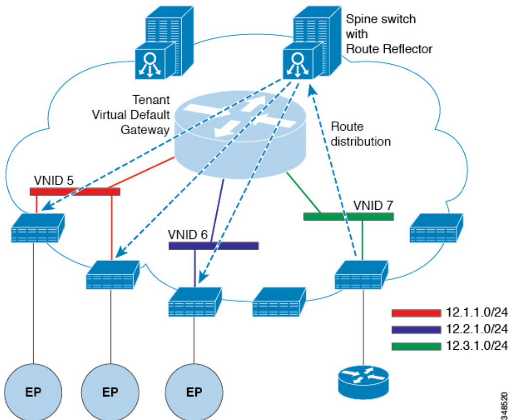
Figure 24: Router Peering
