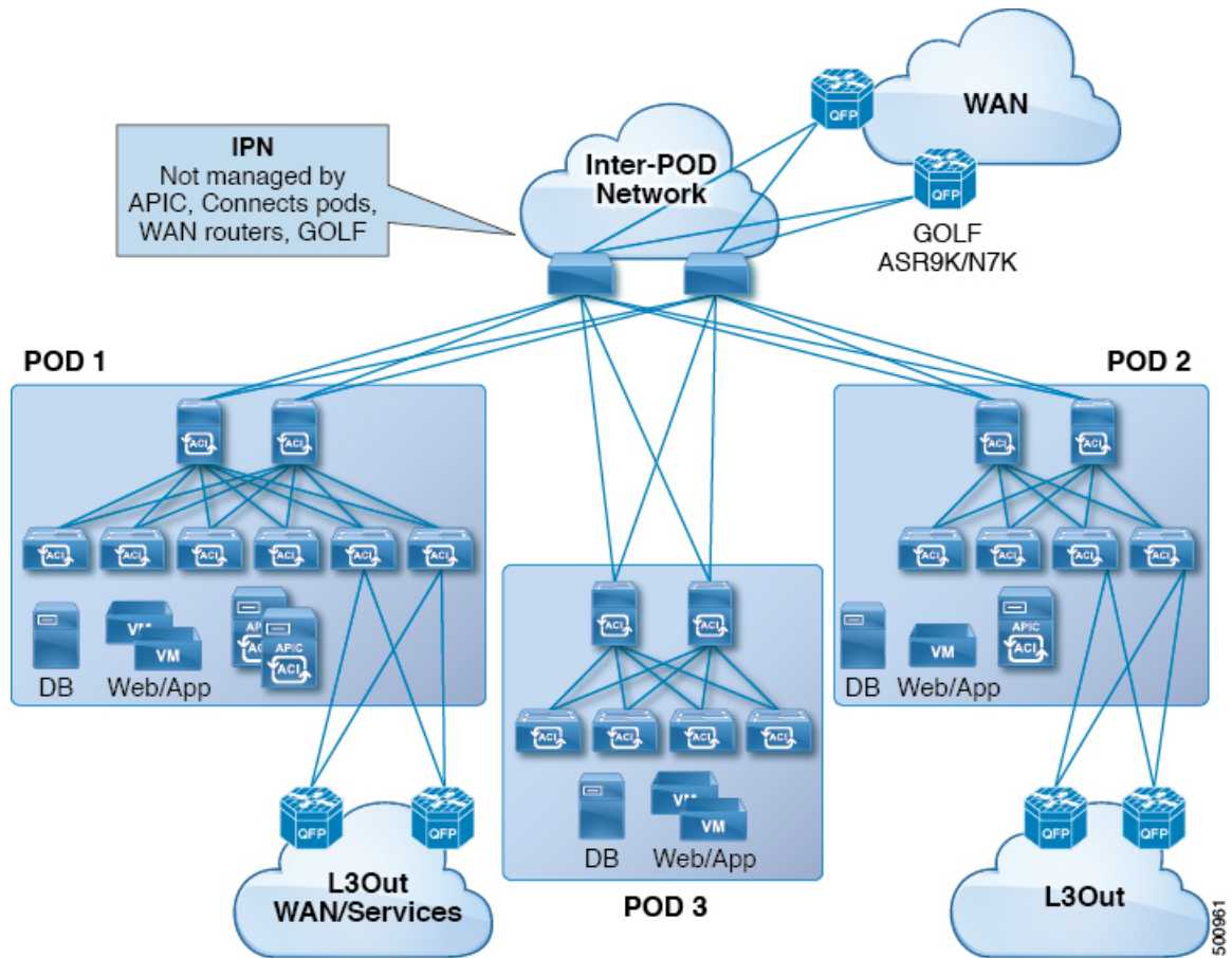
Figure 10: Multi-Pod Overview
