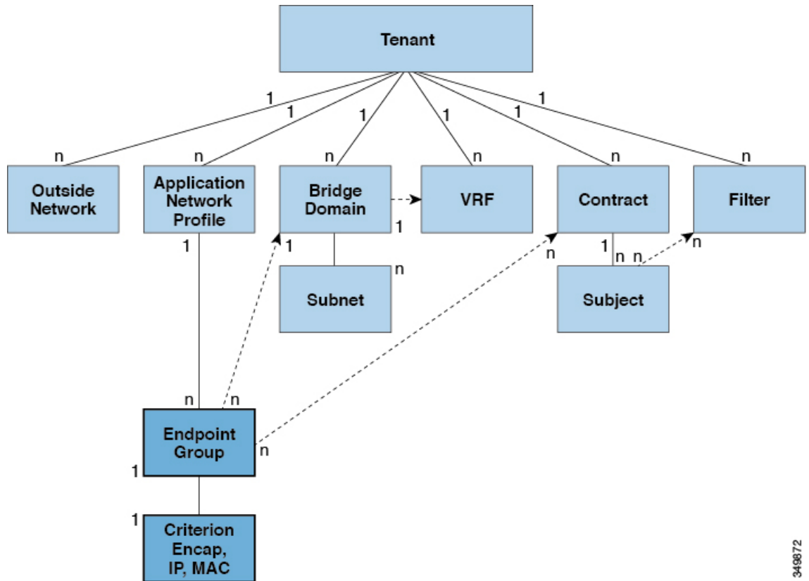
Figure 6: Endpoint Groups
