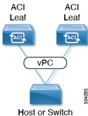
Figure 11: vPC Domain
