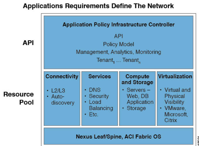
Figure 1: APIC Overview
