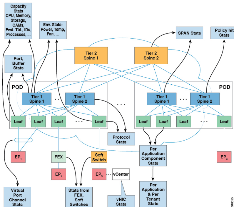
Figure 126: Various Sources of Statistics
