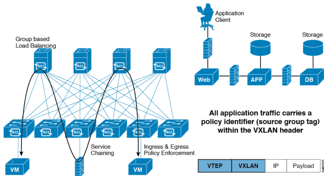
Figure 44: Policy Identification and Enforcement
