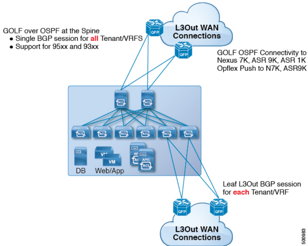
Figure 74: Cisco ACI GOLF Topology
