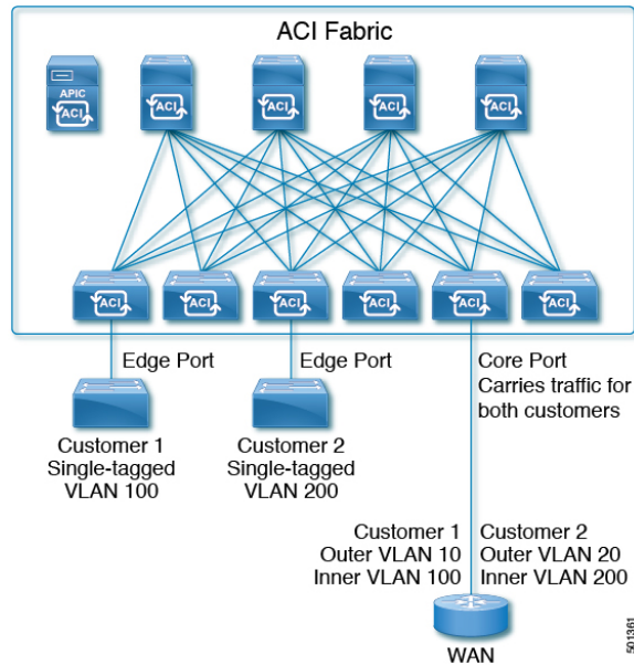
Figure 14: ACI 802.1Q Tunnels
