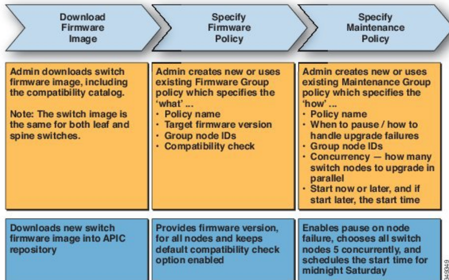
Figure 17: Switch Firmware Upgrade Process
