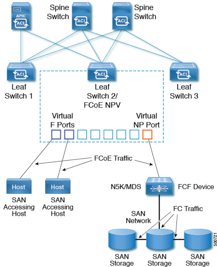
Figure 13: Cisco ACI Topology Supporting FCoE Traffic
