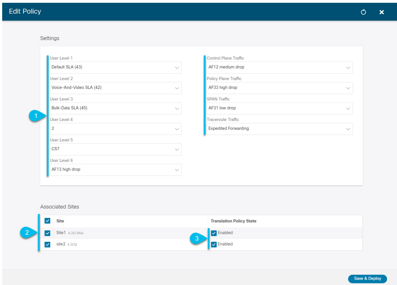
Figure 2. Update the global DSCP policy
