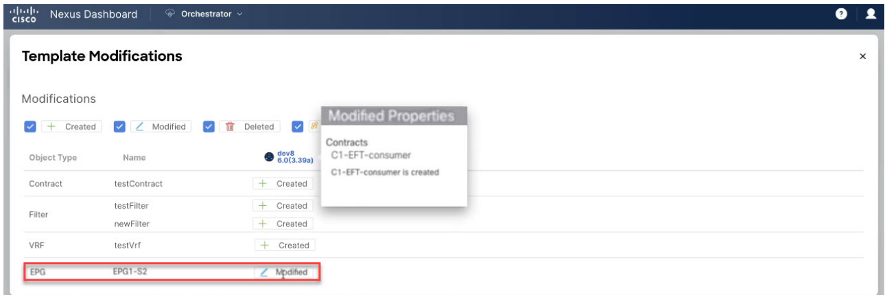
Figure 4. Template Status
