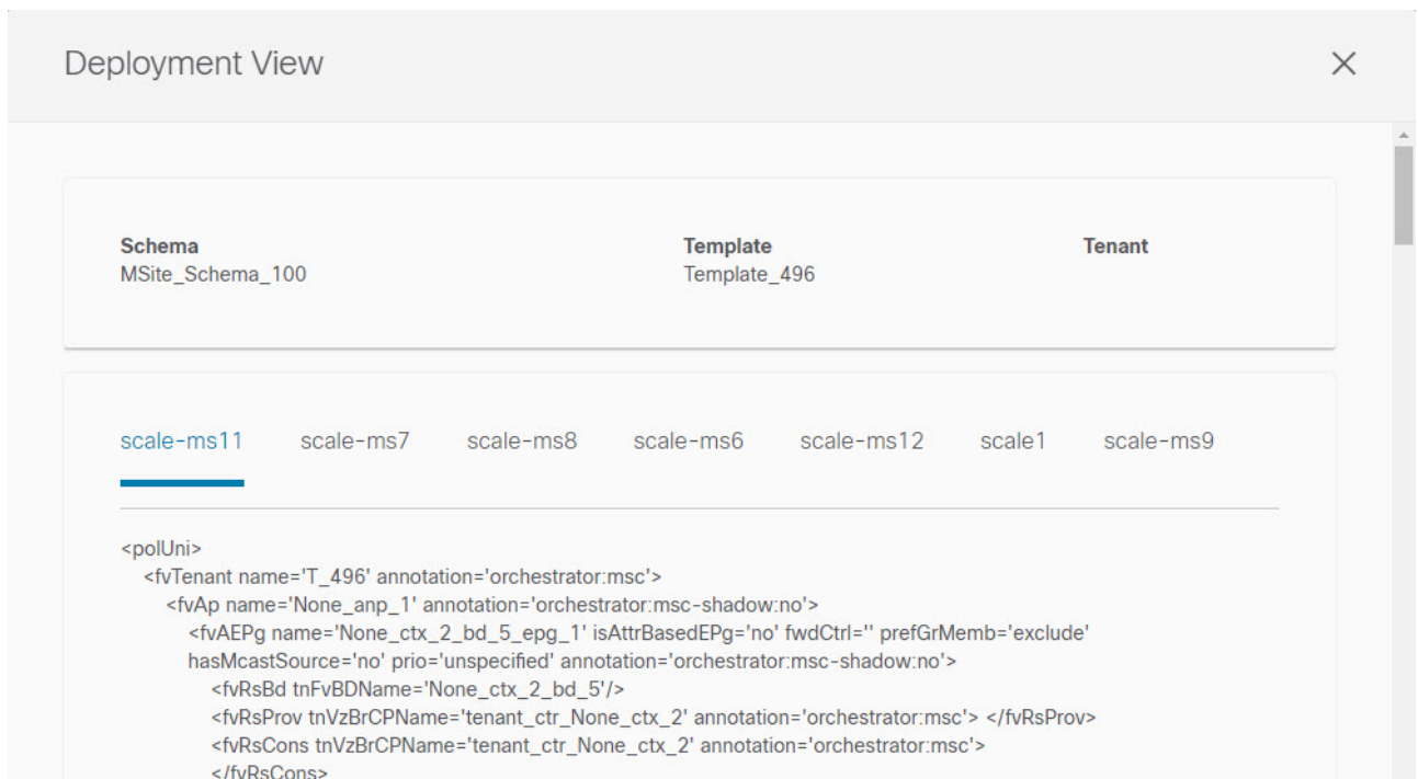
Figure 11. Deployment View
