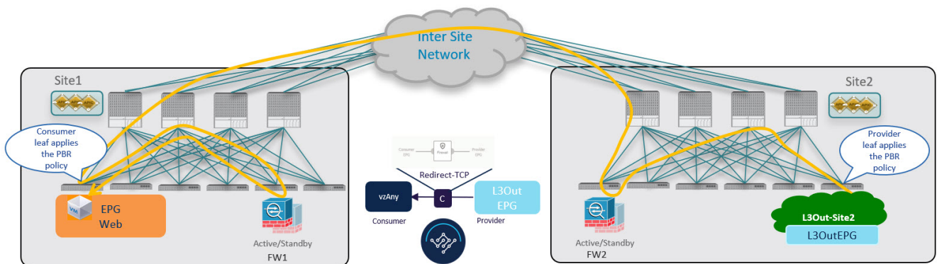
Figure 13. vzAny-to-L3Out Provider-to-Consumer Traffic Flow
