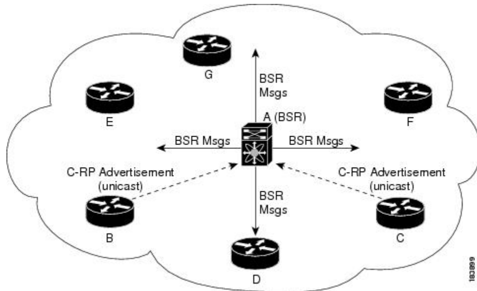
Figure 9: BSR Mechanism
