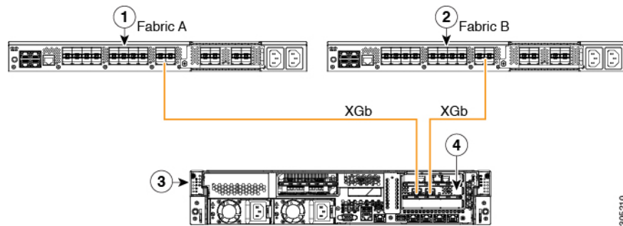
Figure 11: Direct Connect Cabling Configuration with Cisco VIC 1455
